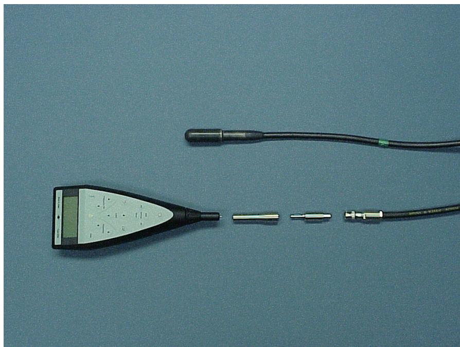
Figure 2. The USLM system unassembled with all the components shown. The components are laid out in the configuration in which they will be used for assembly. The user should familiarize themselves with each component prior to assembly. A cylindrically shaped calibrator for the USLM hand-held system is also enclosed (not shown).
