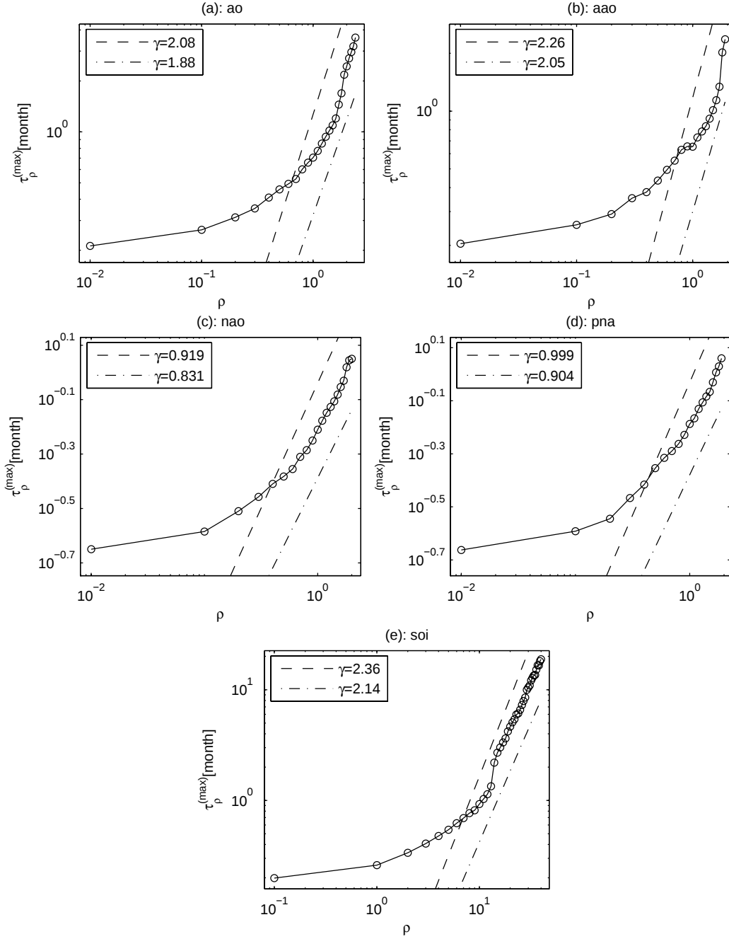
Figure 7. Dependence of the optimal FPT, \tau_{\rho}^{(max)} , on the index reduction \rho for (a) Arctic Oscillation (AO), (b) Antarctic Oscillation (AAO), (c) North Atlantic Oscillation (NAO), (d) Pacific/North American Pattern (PNA), and (e) Southern Oscillation (SO). Power-law exists for large \rho values.
