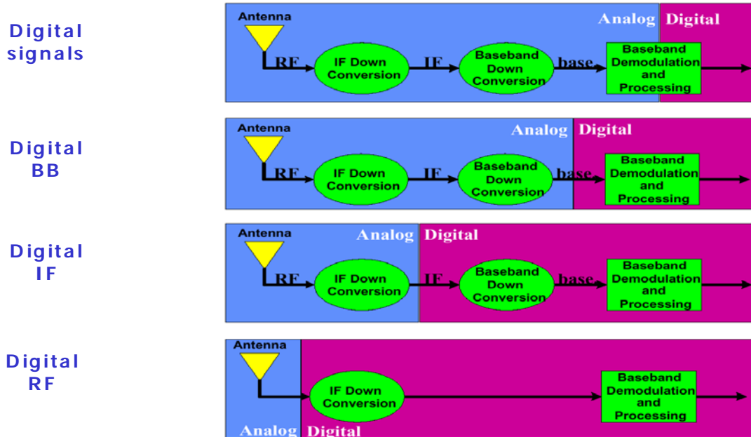
Figure 5: Implementation levels
