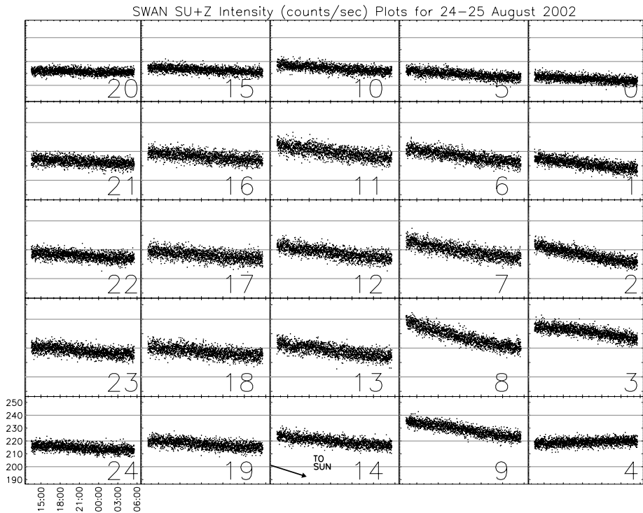
Figure 3 Intensity (counts/s) vs. time plots of 25 SU+Z sensor pixels for SWAN observing period on 24–25 August 2002. SWAN SU+Z was located at 122 R_S and 85^\circ . These plots are positioned to correspond to SU+Z pixel locations and the arrow shows the line towards the Sun given the sensor configuration shown in Figure 2.
