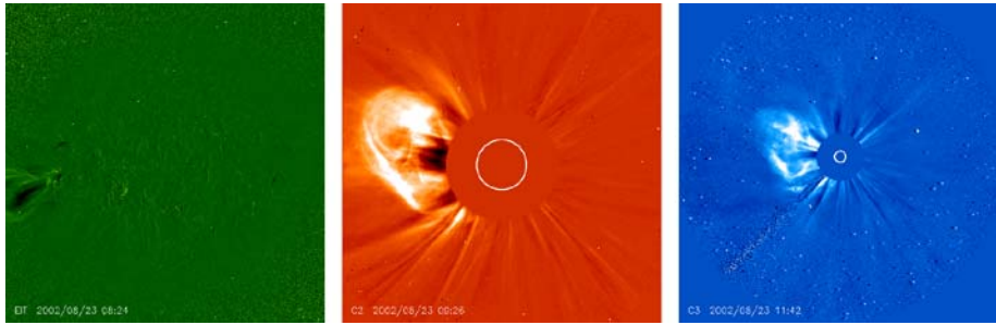
Figure 7 EIT (Fe XII 195 Å), shown on left), LASCO C2 (field-of-view 1.5 to 6 R_{\odot} , shown in middle), and LASCO C3 coronagraph (field-of-view 3.7 to 30 R_{\odot} , shown on right) for the 23 August 2002 08:26 UT CME. The white circle in the LASCO frames shows the relative size and location of the solar disk.
