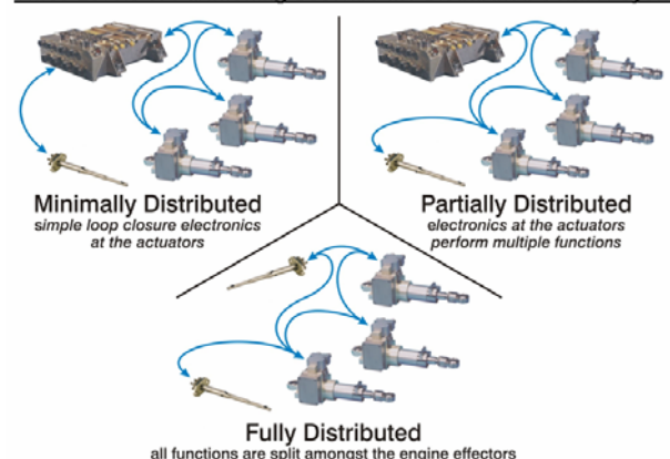
Figure 3: Functional partitioning is shown at three different levels in DCS (HiTEC)
