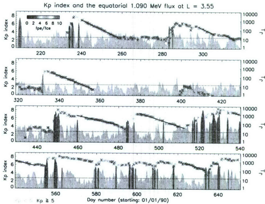
Figure 1. The K_p index and the equatorial perpendicular differential number flux of 1.09 MeV electrons at L = 3.55 as a function of day number for the entire CRRES mission. The K_p index has been smoothed using a 15-hour running mean and the data points are color-coded according to the value of f_{pe}/f_{ce} at the time of the measurement. The K_p value of 3^- is represented by the horizontal dashed line. The best fits to the selected decay periods are overplotted on the data.
