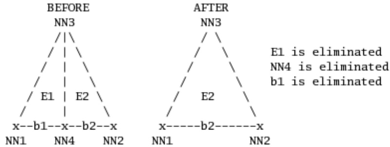
Figure 28. Sketch of the merge 2 boundary elements operation on two hypothetical boundary elements. On the left are two adjacent boundary elements (E1 and E2), while on the right is shown the merged boundary element (E2). Identified are the eliminated boundary element (E1), boundary node (NN4), and boundary edge (b1).
