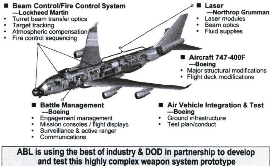
Figure 1. Airborne Laser Weapon System Elements
