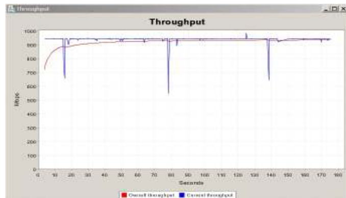
Figure 6.8 – The throughput recorded for a 20 GB file transfer. The effective file transfer rate measured over OMNInet was 920 Mbps using ftp .
