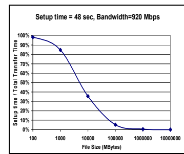
Fig 6.12: Overhead is insignificant at 100 GB
