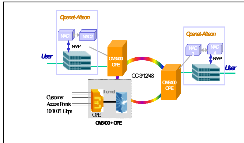
Figure 6.1: Service platform for Dynamic bandwidth allocation over RPR metro network
