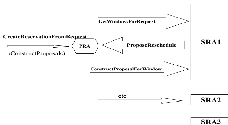
Figure 8.4 – Four-step algorithm.
