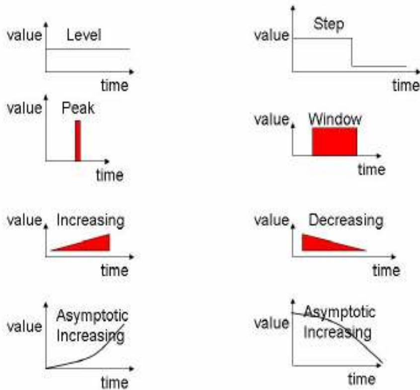
Figure 7.2 - Time-Value Curves.
