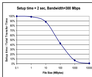
Fig 6.11: Overhead is insignificant at 5 GB
