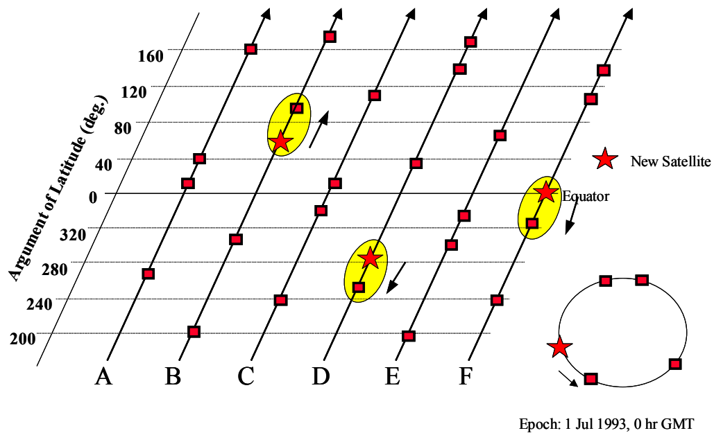
Figure 7. GPS Constellation With 27 Optimized Slots 8
