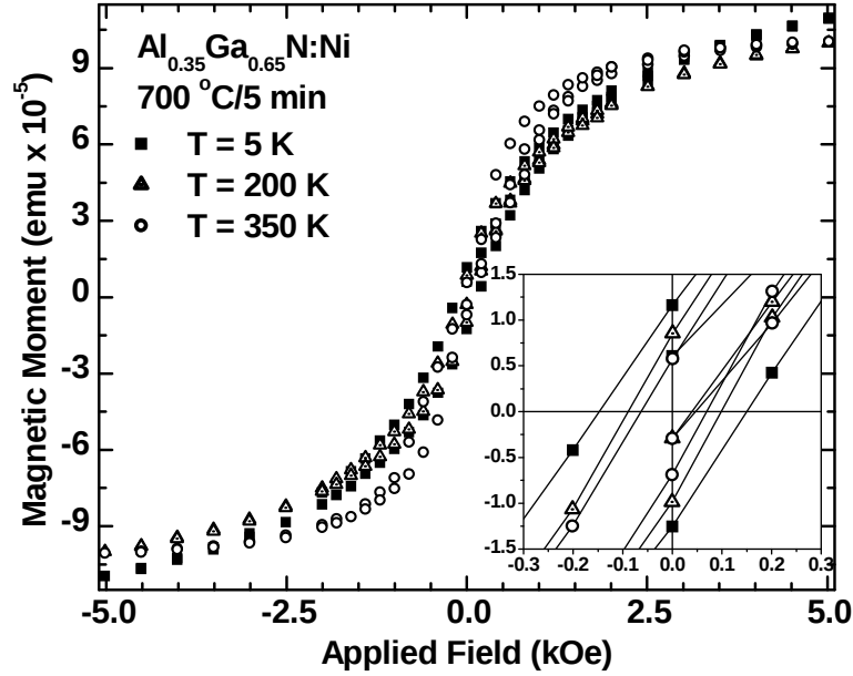
Fig. 3. Variable field measurements taken at temperatures of 5, 200, and 350 K for Ni-implanted \text{Al}_{0.35}\text{Ga}_{0.65}\text{N} annealed at 700 °C for 5 min. The inset is a close-up view of magnetic behavior near the origin to show the effect of temperature on remanent and coercive field strengths.
