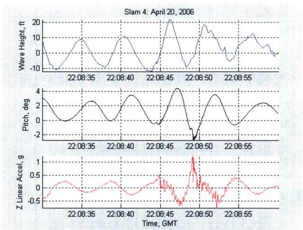
Figure 40. Slam Event 4: 30 second close up plots of slam event.
