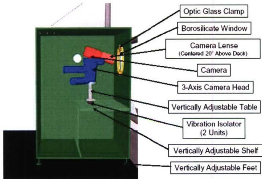
Figure 17. Camera mount arrangement.
