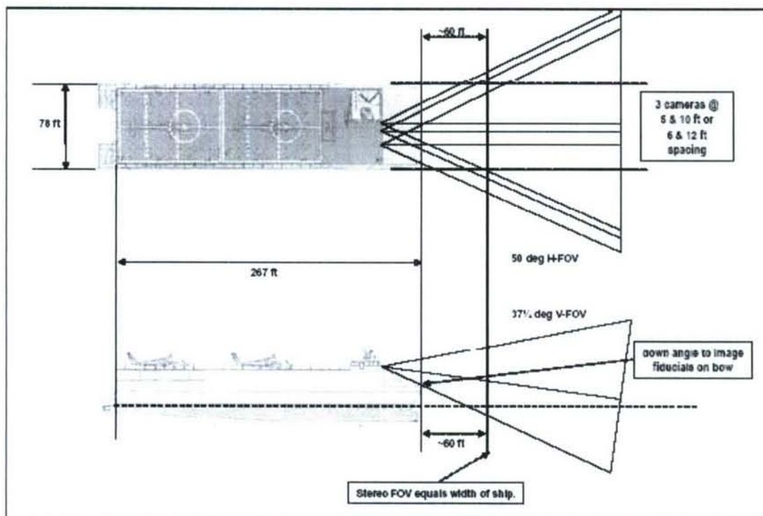
Figure 15. Sea Fighter Imaging Geometry.
