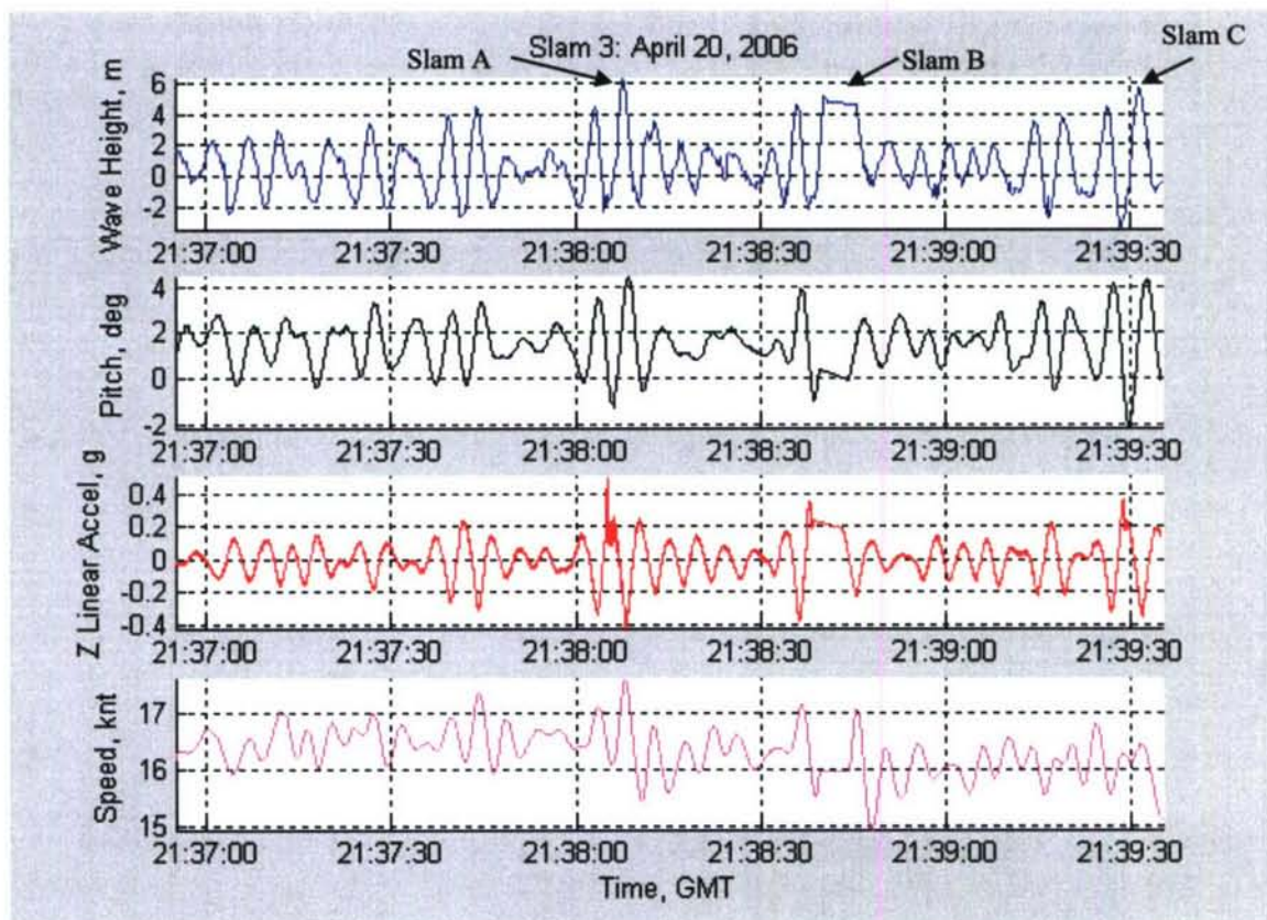
Figure 33. Slam Event 3: Wave Height, Pitch, Vertical Acceleration, and Speed plots.
