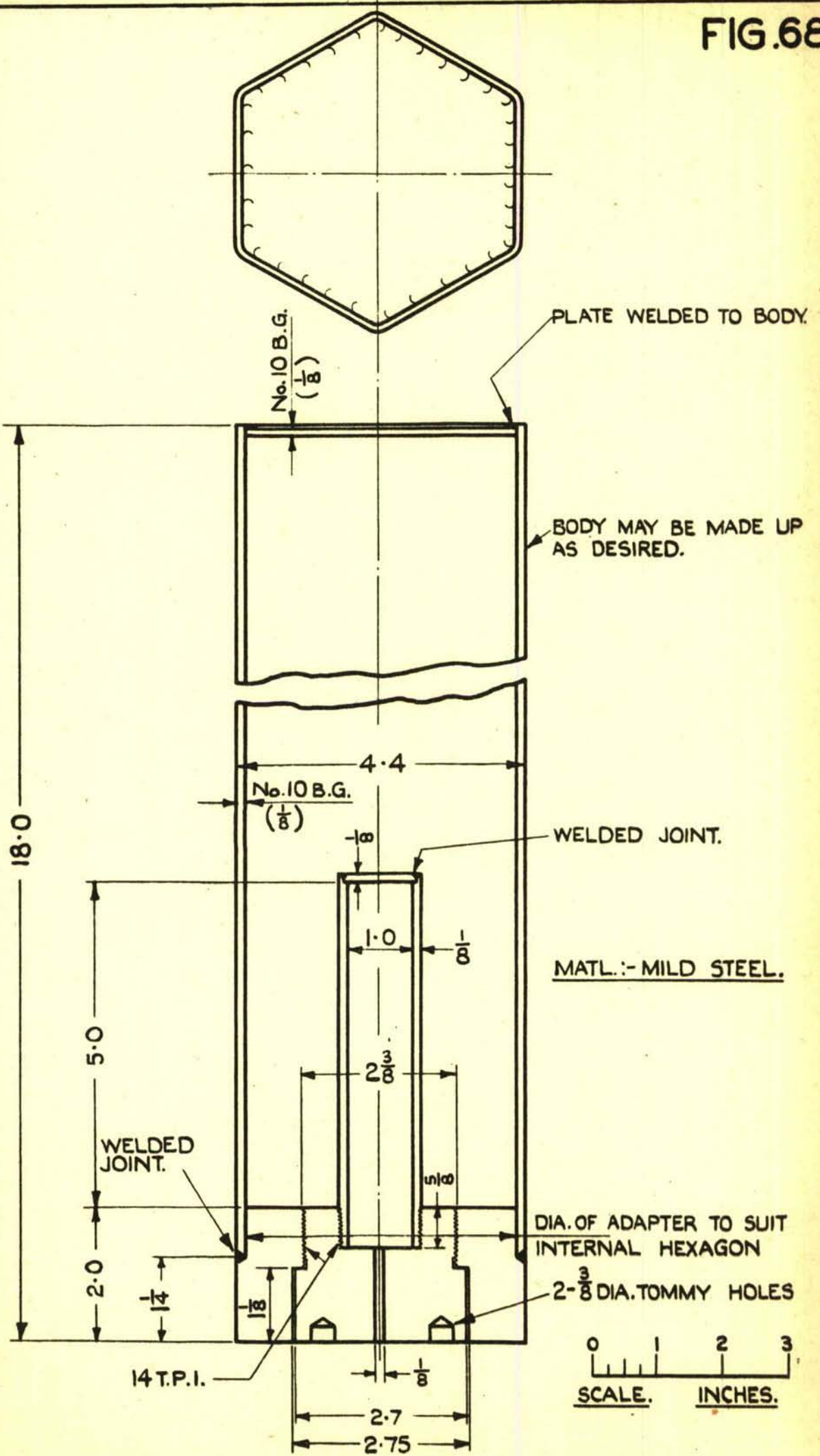
25 LB. HEXAGONAL INCENDIARY BOMB.
