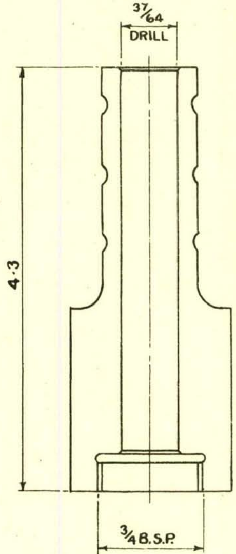
ALTERNATIVE NOSE-STEEL "B"
