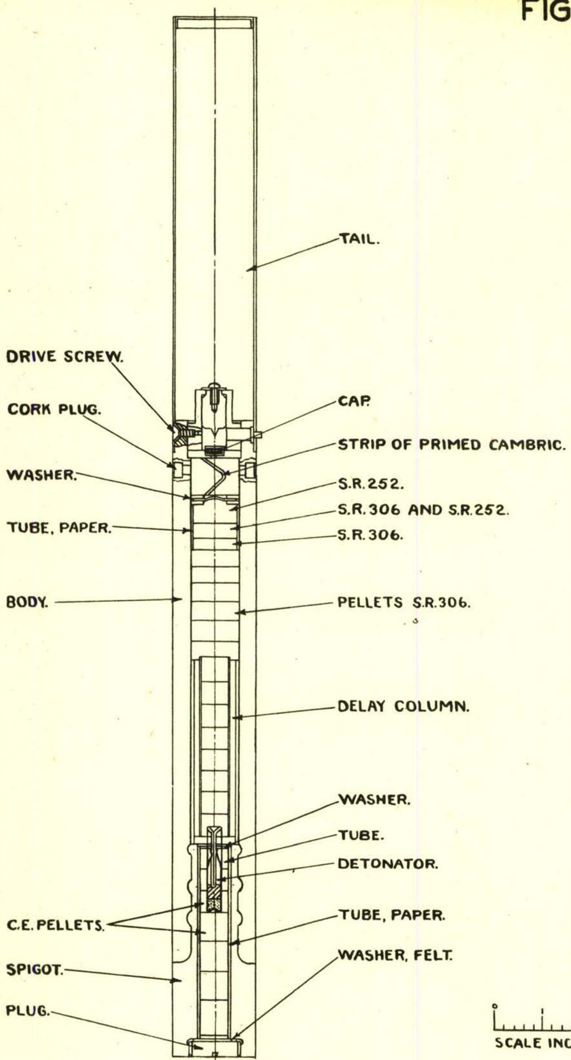
BOMB, INCENDIARY, A/C. X. 4LB. MK. 3.
