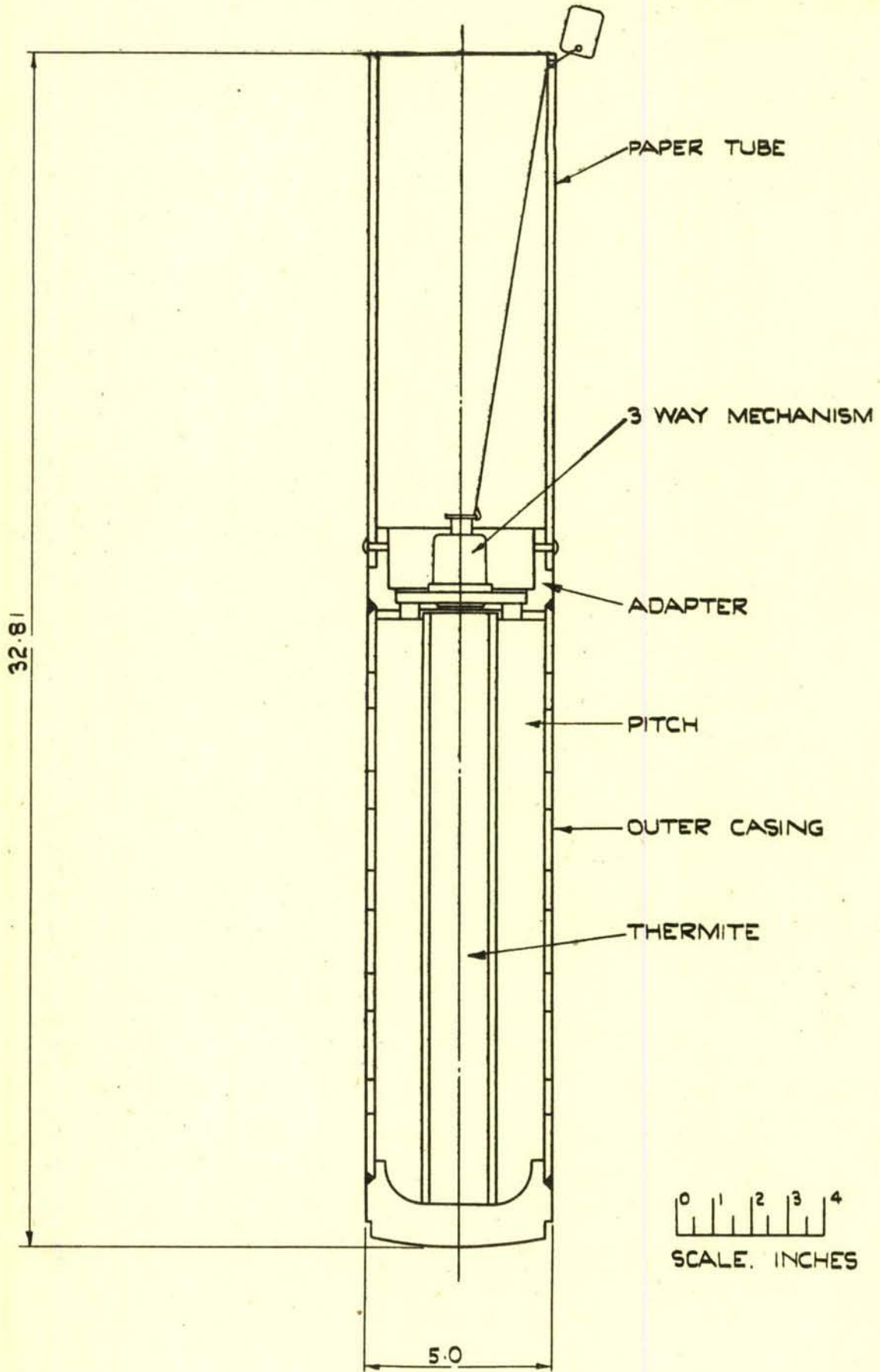
BOMB. INCENDIARY. A/C 37 LB. FILLED THERMITE & PITCH.
