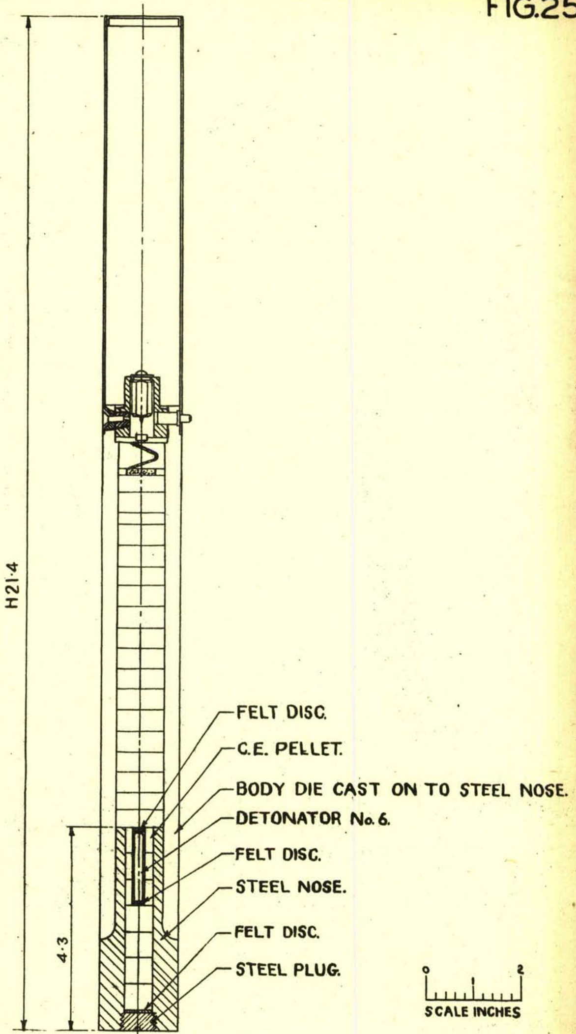
BOMB, INCENDIARY, A/C, 4LB. X TYPE.
