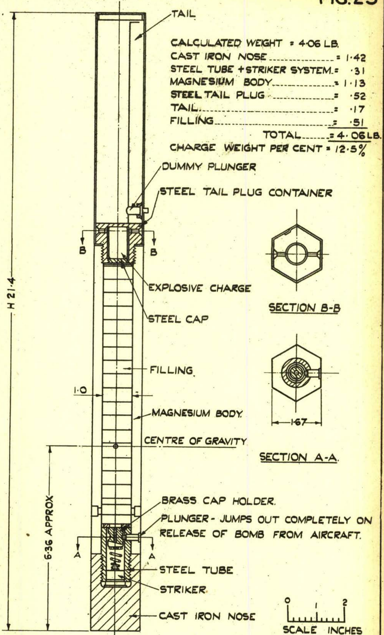
BOMB, INCENDIARY, A/C. 4 LB. X TYPE.
