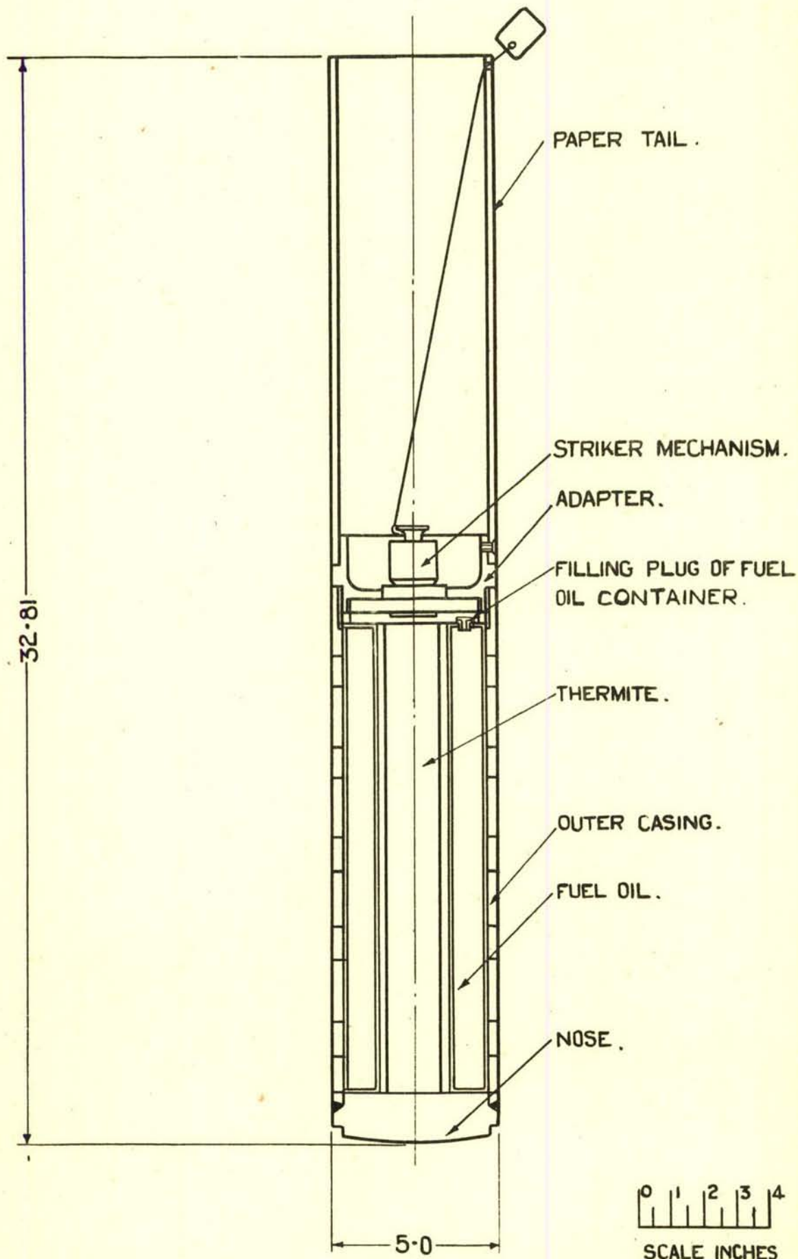
BOMB, INCENDIARY, A/C. 40 LB. FILLED FUEL OIL & THERMITE.
