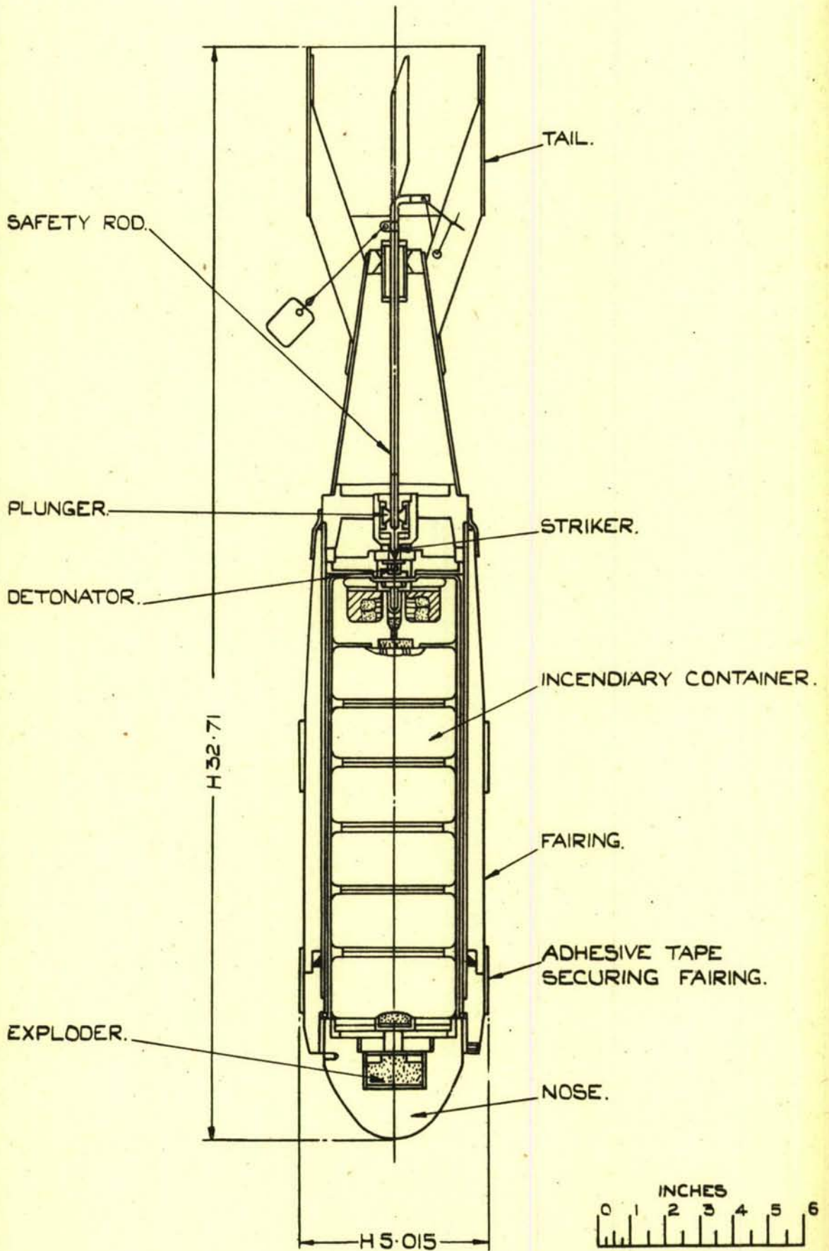
BOMB, INCENDIARY, A/C 40 LB. MK. I.
