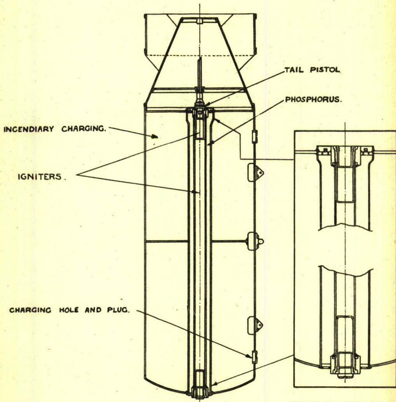
ENLARGED VIEW OF ENDS OF CENTRAL TUBE.
