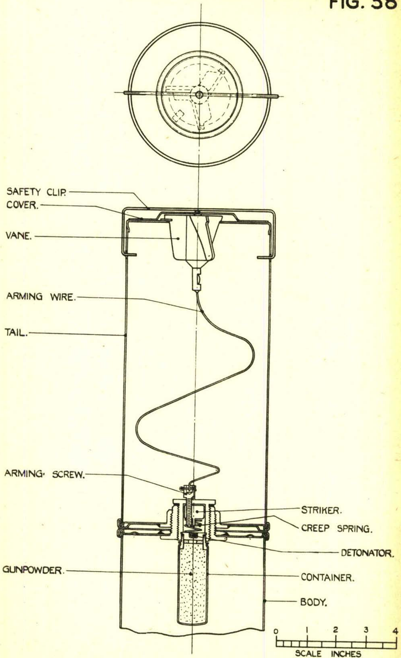
IGNITER FOR BOMB A/C L.C. 30LB. MKII
