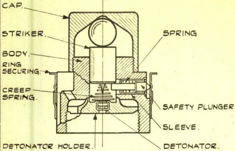
SECTION THRO' C
