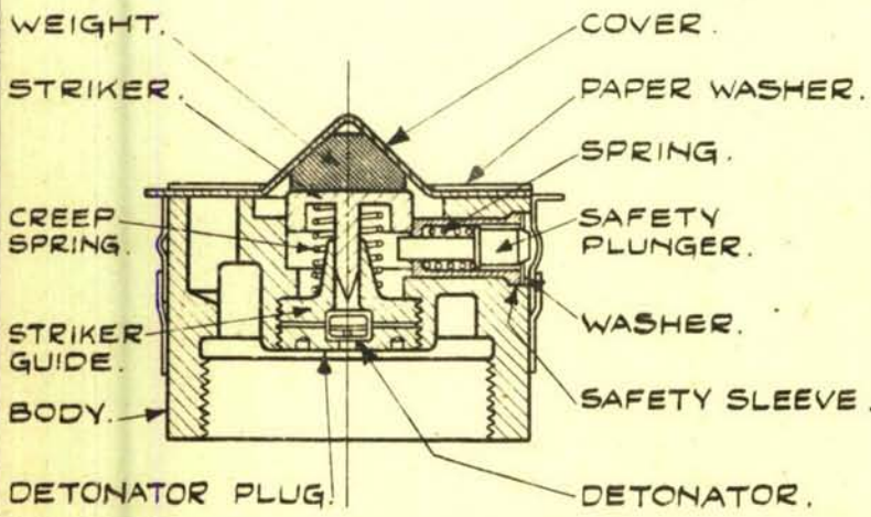
FUZE BASED ON DRG. No. D.D.(L)14870, A.
