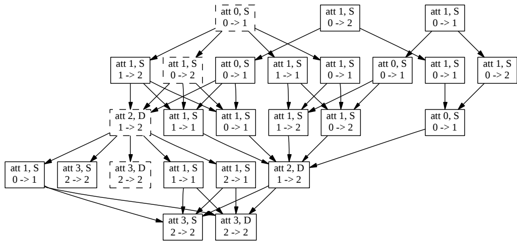
Figure 4: Attack Graph
