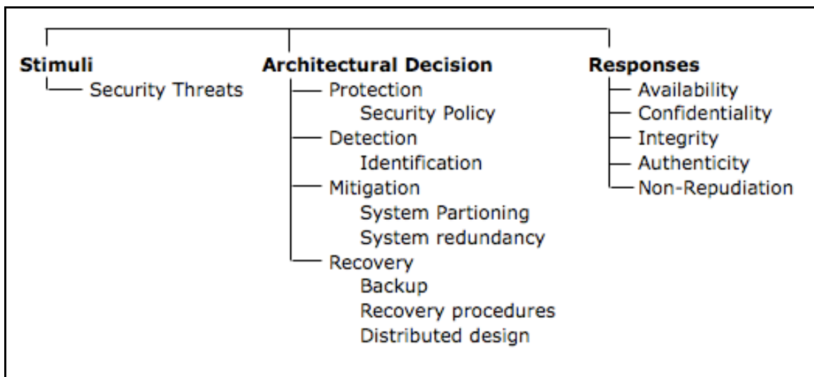
Figure 4. Security Characterization
