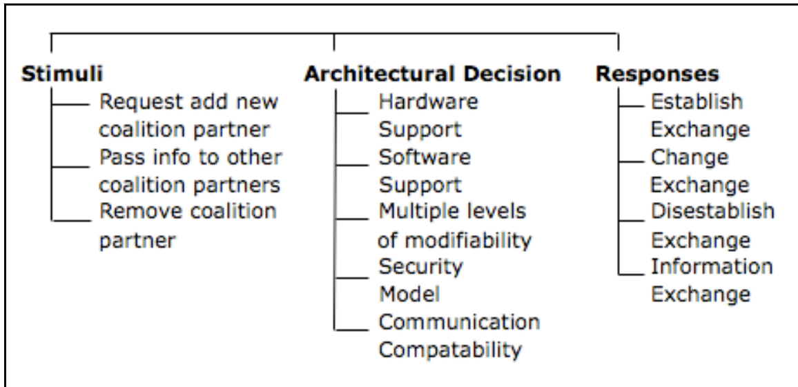
Figure 2. Modifiability Characterization
