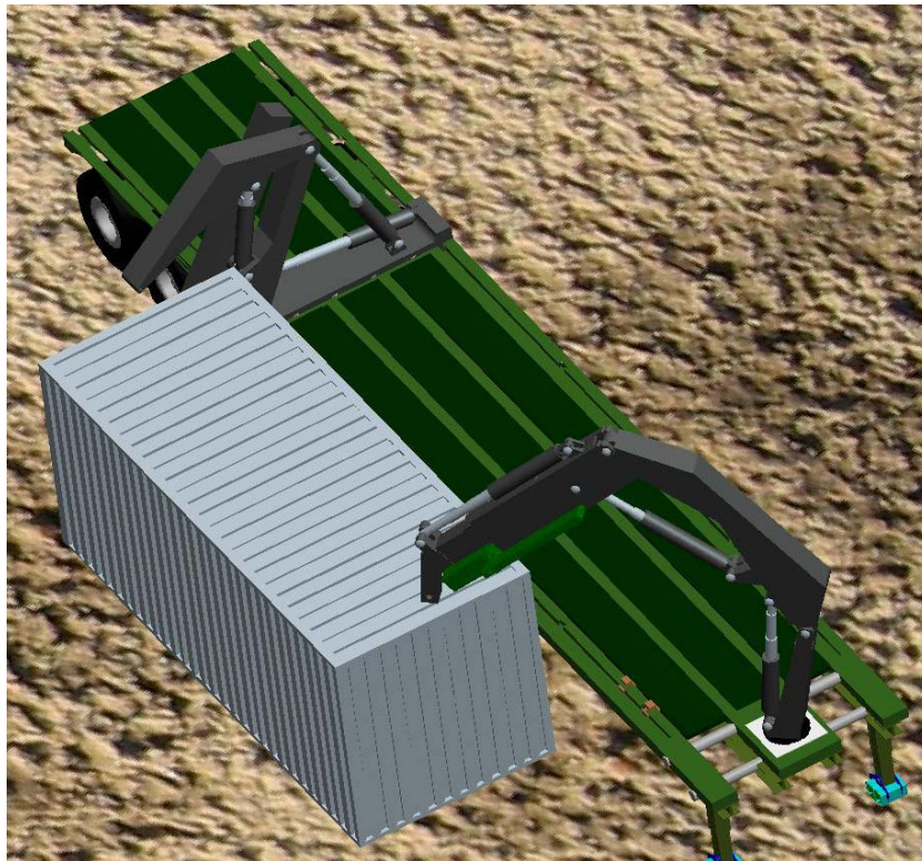
Figure 1: Best Technical Approach, MFT with Side-loading Crane & Smart Crane
