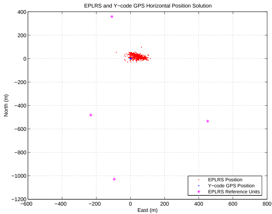
Figure 9: V1 EPLRS Position Error with 4 reference units
