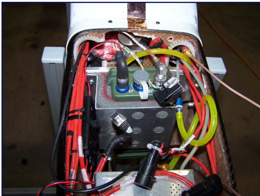
Figure 2: EPLRS Micro-Light installed in UAV
