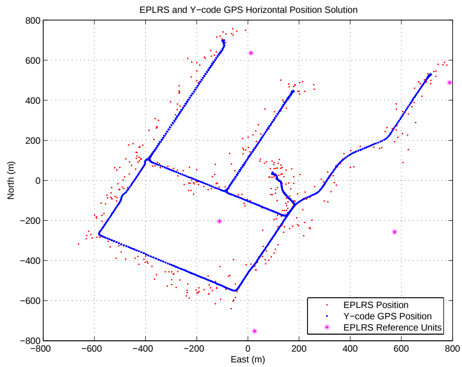
Figure 16: Dynamic Tests with 5 reference RS units
