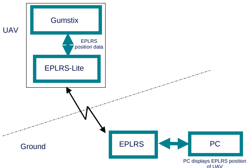
Figure 4: Proposed Air-to-Ground Communications over EPLRS for EPLRS Position
