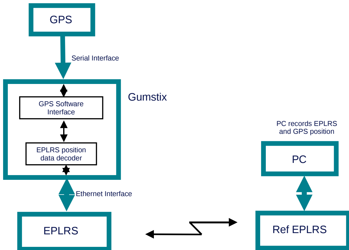
Figure 6: EPLRS and Gumstix Test Setup
