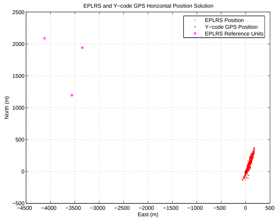
Figure 15: 4 km offset EPLRS Position Error with 3 reference units
