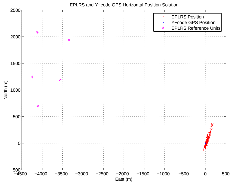
Figure 13: 4 km offset EPLRS Position Error with 5 reference units
