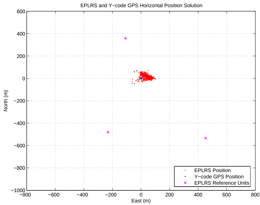
Figure 10: V1 EPLRS Position Error with 3 reference units
