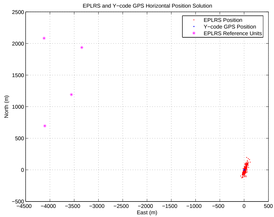
Figure 14: 4 km offset EPLRS Position Error with 4 reference units
