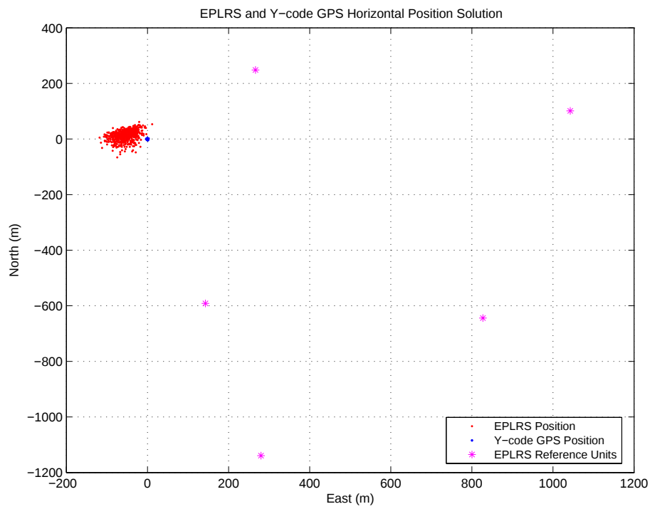
Figure 12: V3 EPLRS Position Error with 5 reference units
