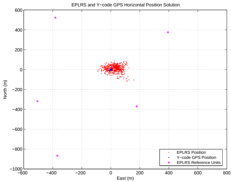
Figure 11: V2 EPLRS Position Error with 5 reference units
