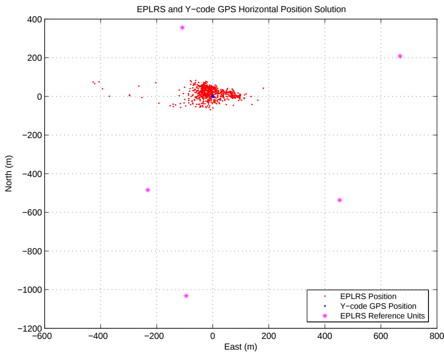
Figure 7: V1 EPLRS Position Error with 5 reference units (1 of 2)
