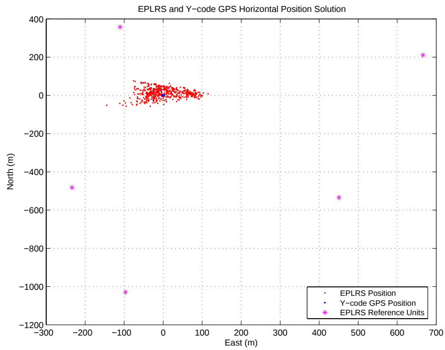
Figure 8: V1 EPLRS Position Error with 5 reference units (2 of 2)
