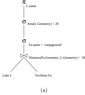
Figure 6: SQL query tree
