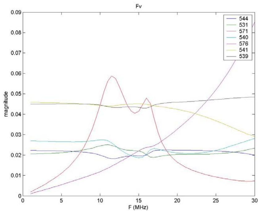
Figure 33 Eigencurrent amplitudes of the Macchi model when exposed to V-polarised plane waves from the front. Note that amplitudes are \sim 20 dB less than for H polarised waves. Wing currents (#572, #573) are barely excited.
