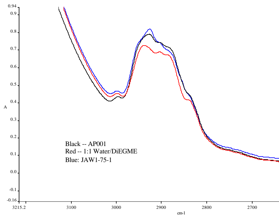
Figure 53. FT-IR Spectra of Thin Apple Jelly, DiEGME/Water, and JAW1-75-1 (2700 - 3215 \text{cm}^{-1} )
