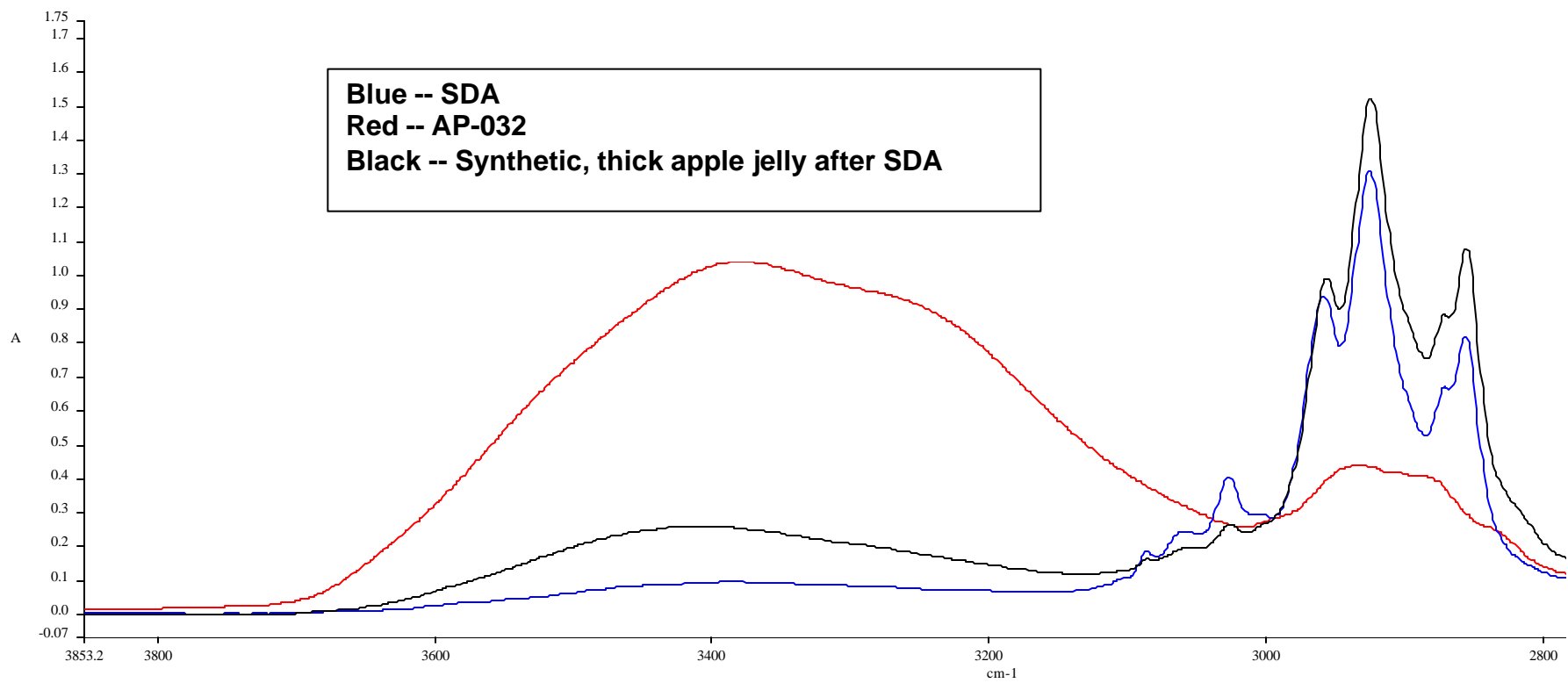
Figure 67. FT-IR Spectra of SDA, Thick Apple Jelly, and Synthetic Thick Apple Jelly (2800 to 3800 cm -1 )
