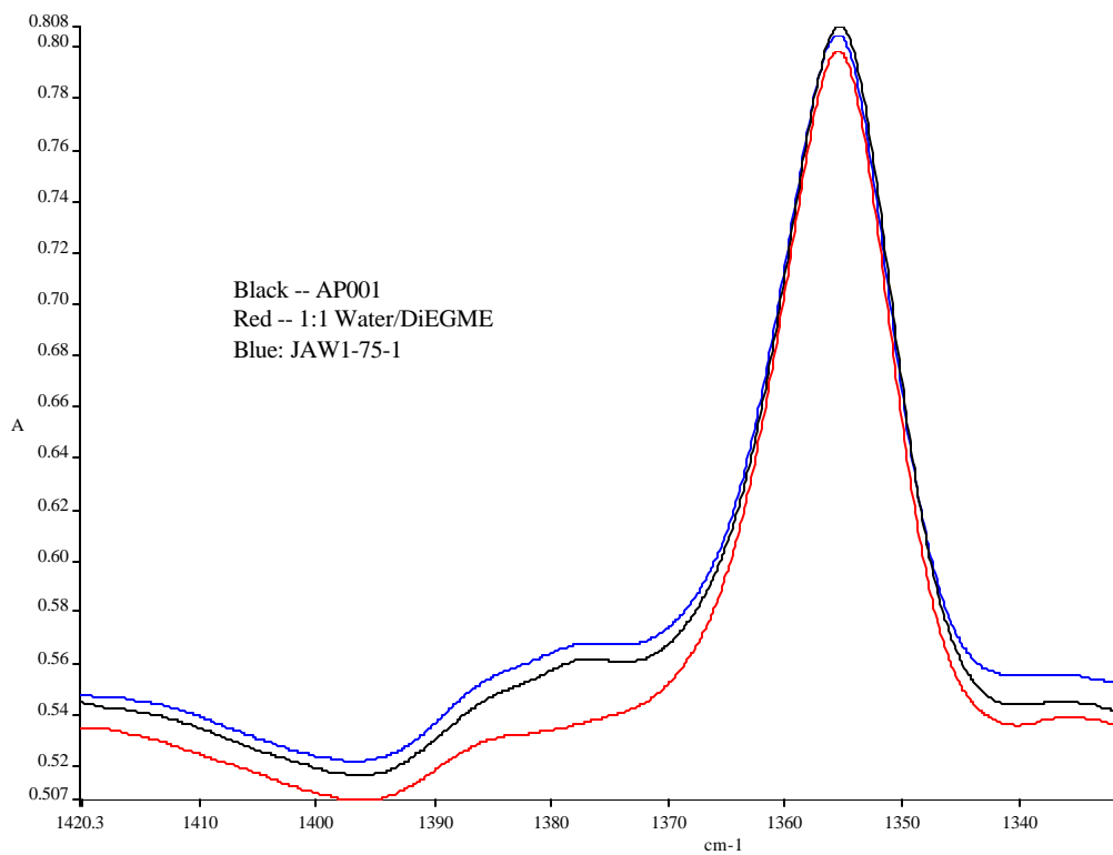
Figure 54. FT-IR Spectra of Thin Apple Jelly, DiEGME/Water, and JAW1-75-1 (1330 - 1420 \text{cm}^{-1} )
