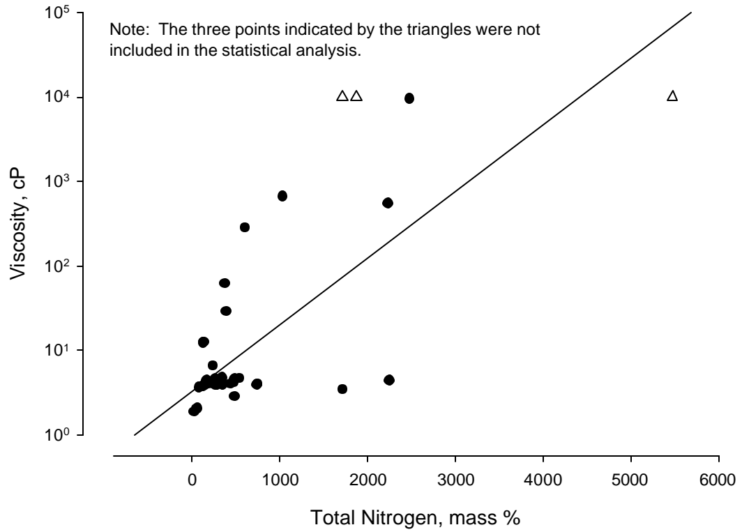
Figure 25. Total Nitrogen vs. Viscosity for Apple Jelly Samples ( R^2=0.37 )
