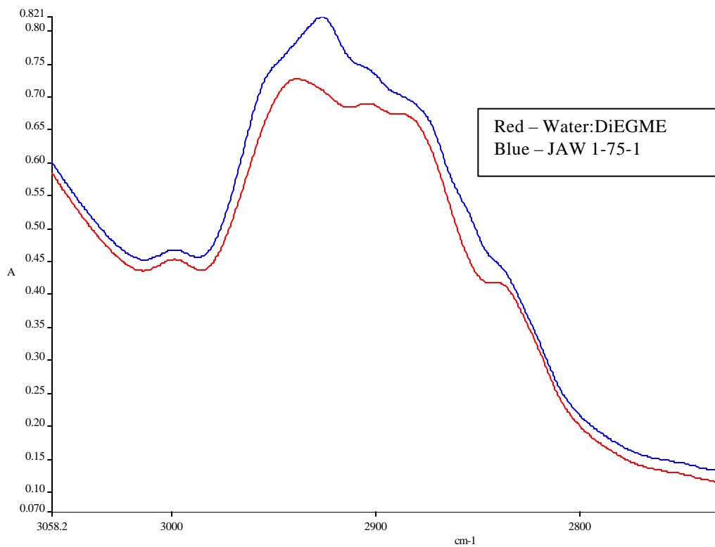
Figure 50. FT-IR Spectra of DiEGME/Water and JAW1-75-1 (2700 - 3058 \text{cm}^{-1} )
