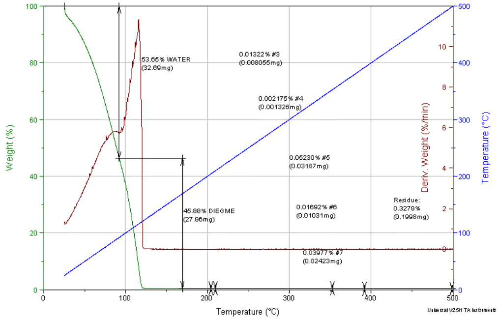
Figure 35. TGA Scan of AP-002 -- Thin
