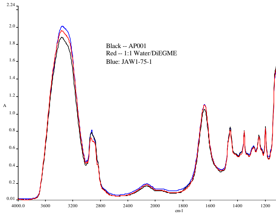
Figure 52. FT-IR Spectra of Thin Apple Jelly, DiEGME/Water, and JAW1-75-1 (1200 - 4000 \text{cm}^{-1} )
