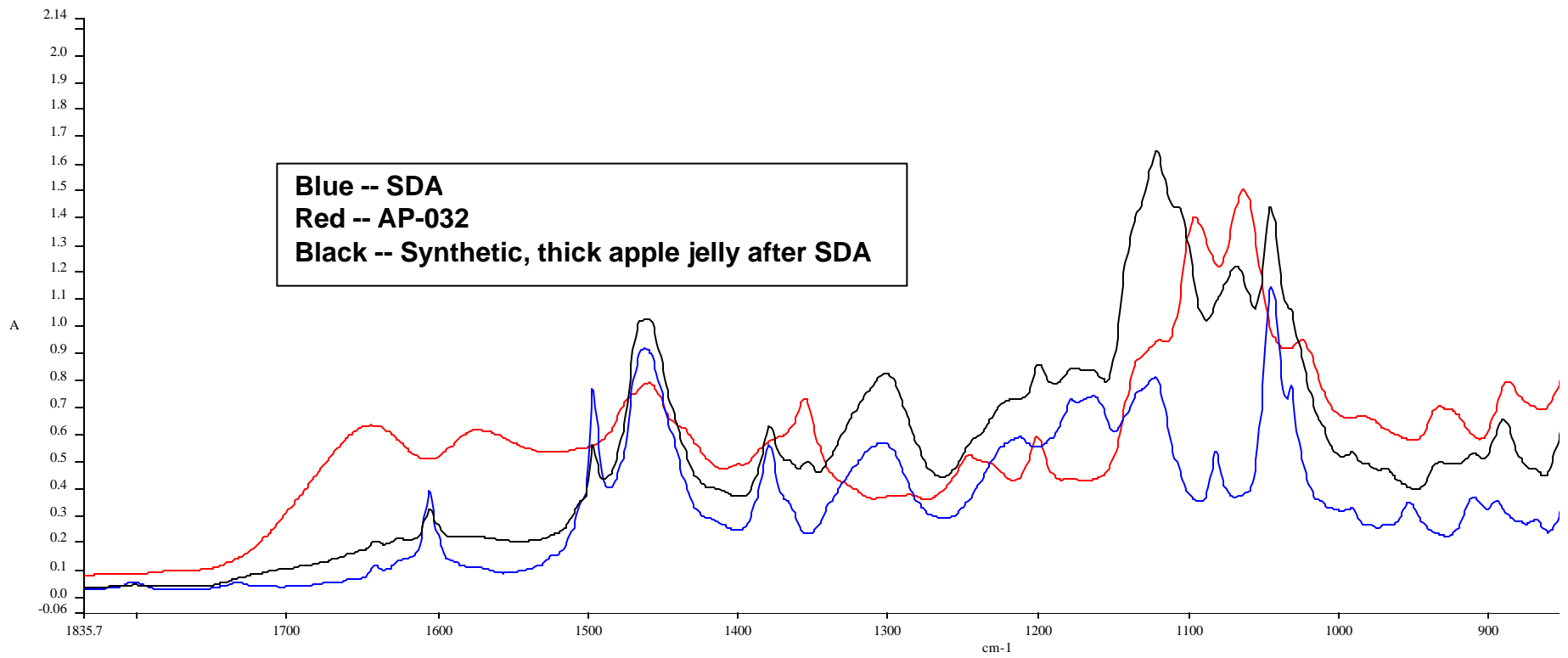
Figure 68. FT-IR Spectra of SDA, Thick Apple Jelly, and Synthetic Thick Apple Jelly (900 to 1800 cm -1 )
