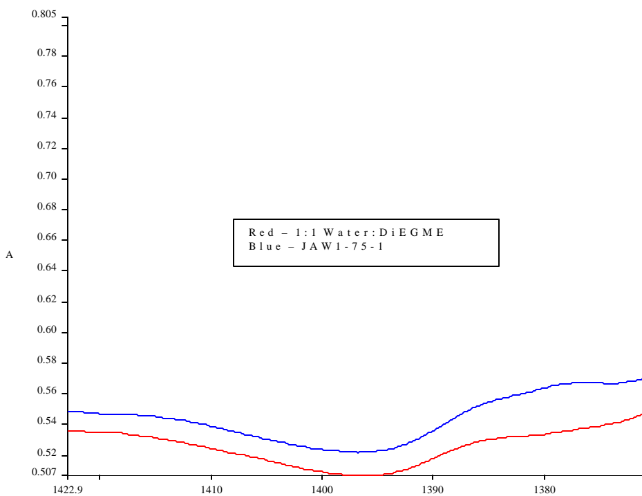
Figure 51. FT-IR Spectra of DiEGME/Water and JAW1-75-1 (1330 - 1420 \text{cm}^{-1} )
