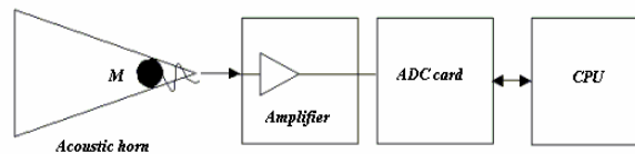
Figure 7: Principal Scheme of a Measurement Channel of Audition Sensors.
