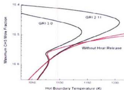
Fig.10. Maximum CH_3 mole fractions as functions of hot air temperatures for 7% CH_4 in N_2 , p=3\text{atm} , a=150\text{ S}^{-1} .
