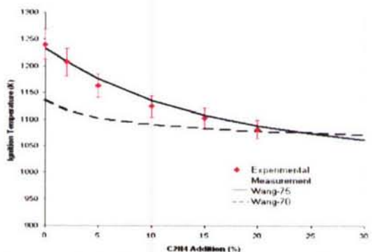
Fig.11. Ignition temperature versus C_2H_4 addition to 20% CH_4 in N_2 , p = 3\text{atm} , strain rate =300\text{ S}^{-1} .
