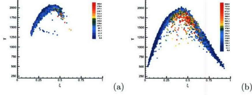
Figure 1: The mean conditionally filtered scalar dissipation conditional on both the mixture fraction and temperature, \langle \chi | \xi, T \rangle_\ell , for \Delta = 3.0mm and \langle \xi \rangle_L = \xi_s at x/D = 7.5 in flame D. The \chi values are given in the legend. (a) \langle \xi''^2 \rangle_L = 0.001 and (b) \langle \xi''^2 \rangle_L = 0.024
