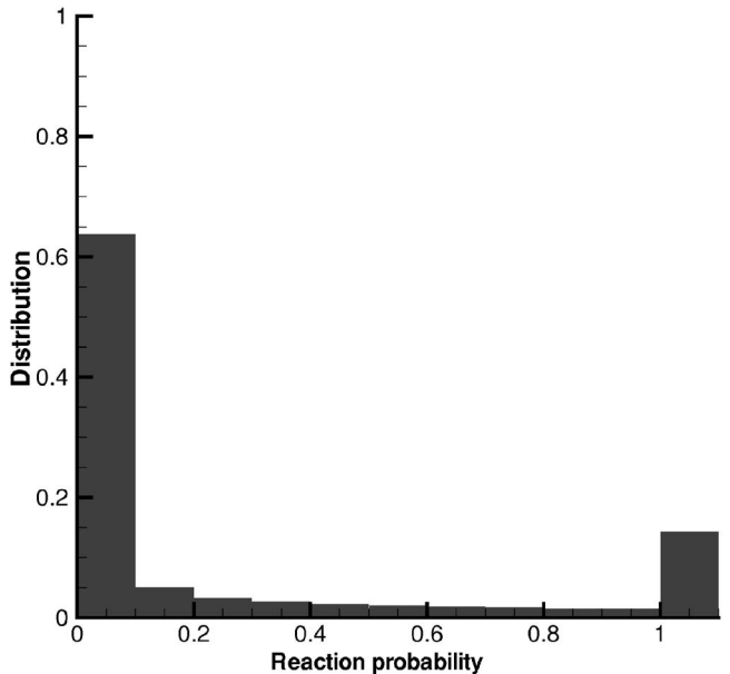
FIG. 3. Reaction probability distribution for \text{O} + \text{HCl} \rightarrow \text{OH} + \text{Cl} using the TCE model (rate constant of Mahmud et al. , Ref. 7) for an altitude of 120 km and a freestream velocity 5 km/s.
