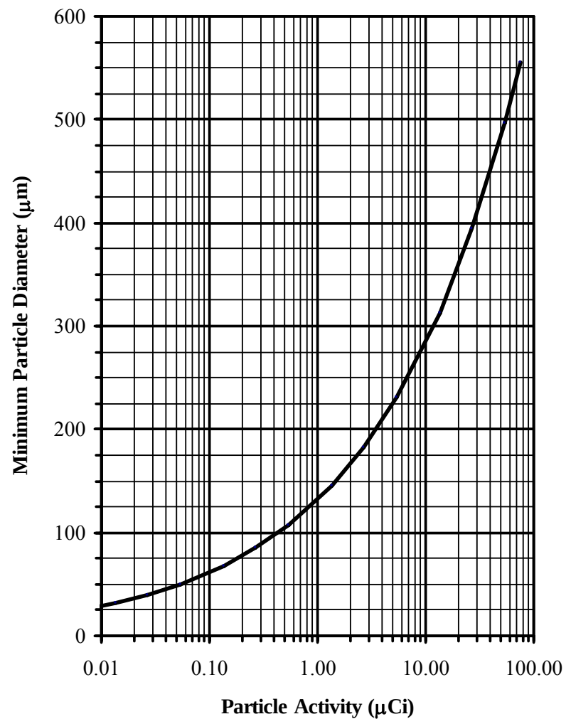
Figure A-9. Minimum ^{239+240}\text{PuO}_2 Particle Diameter, Assuming Spherical, and \rho = 11.5 \text{ g/cm}^3 (High Range).
