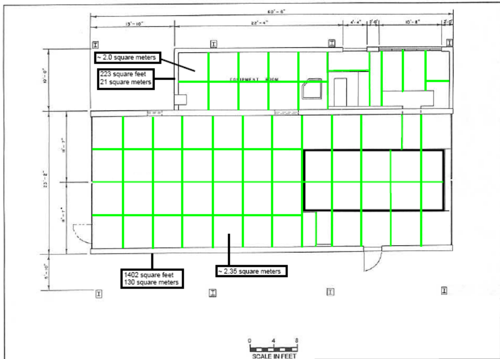
Figure B-2. Example Grid System for Shelter Floor and Pit Surveys.
