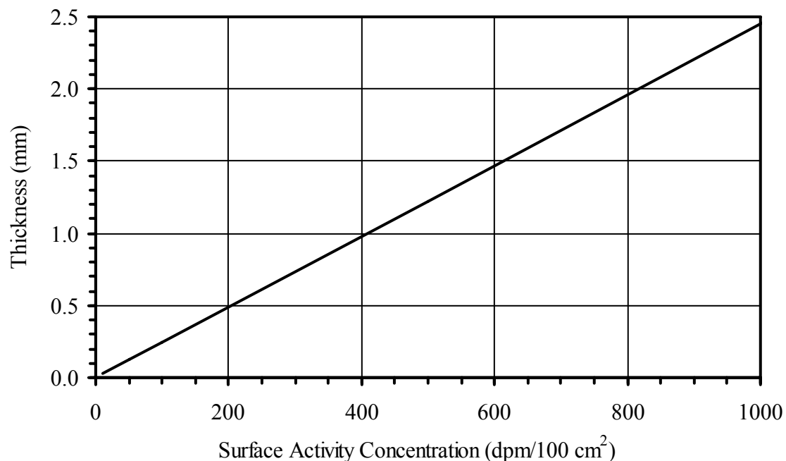
Figure B-1. Averaging Thickness of Concrete vs. Mean Surface Concentrations of 239+240 Pu at 8 pCi/g.
