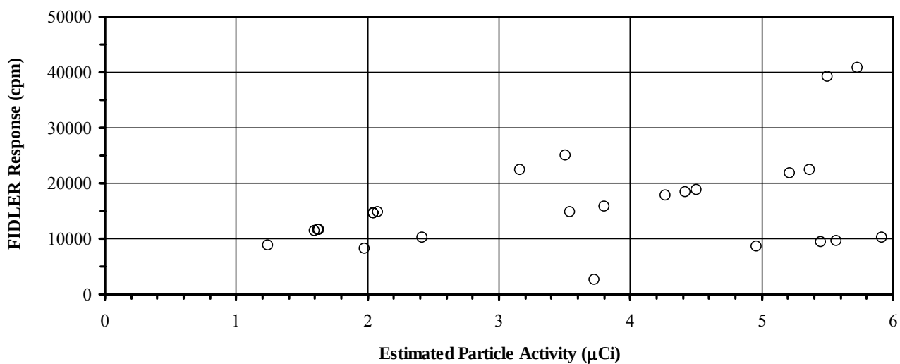
Figure A-16. FIDLER Response vs. Estimated ^{239+240}\text{Pu} Activity [Appendix C, (Cabrera 2006a)].
