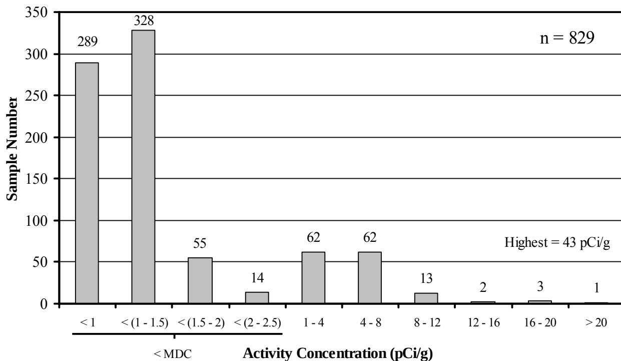
Figure A-12. Systematic Final Status Survey ^{239+240}\text{Pu} Activity Concentration Histogram [Data from Duratek (2006)].
