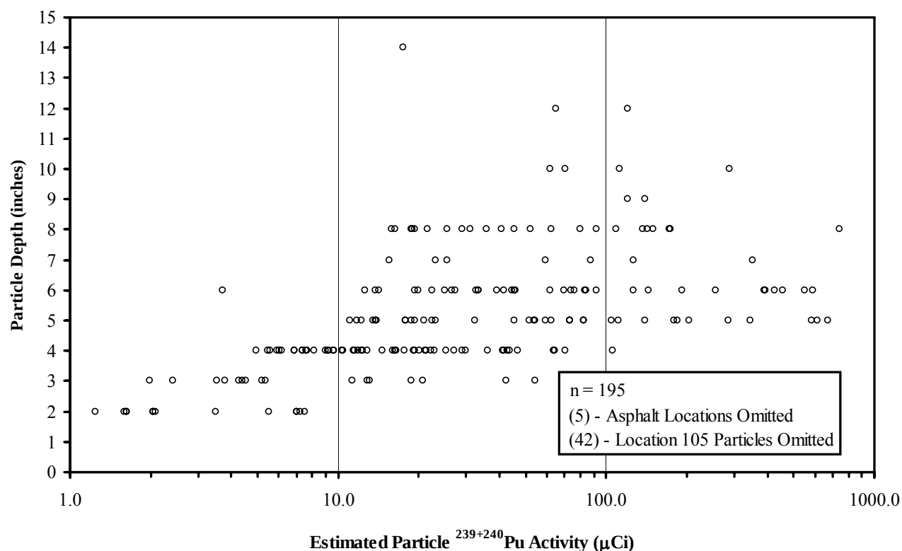
Figure A-15. Estimated Particle ^{239+240}\text{Pu} Activities vs. Depth [Cabrera Services Particle Removal (Cabrera 2006a)].
