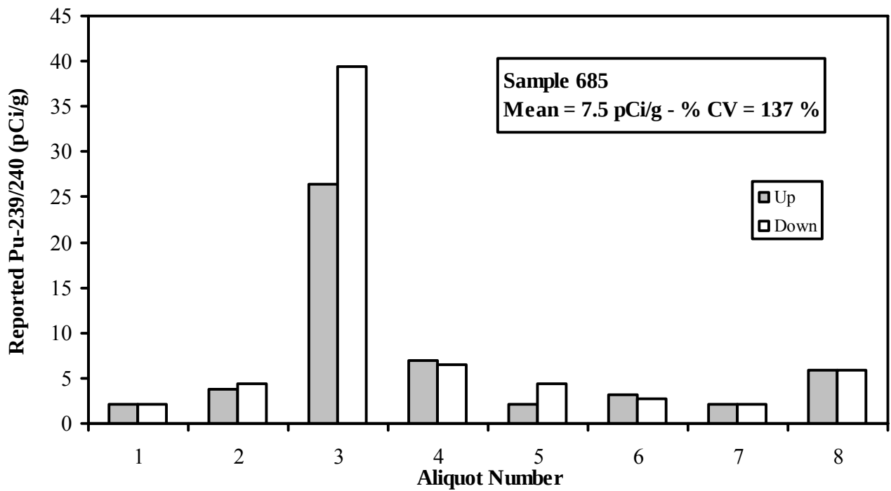
Figure A-6. ^{239+240}\text{Pu} Activity Concentrations of Individual Aliquots (Rademacher 2001).
