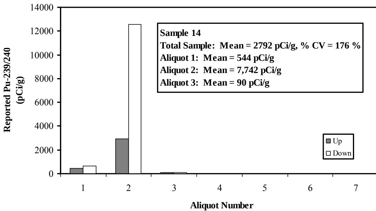
Figure A-5. ^{239+240}\text{Pu} Activity Concentrations of Individual Aliquots (Rademacher 2001).
