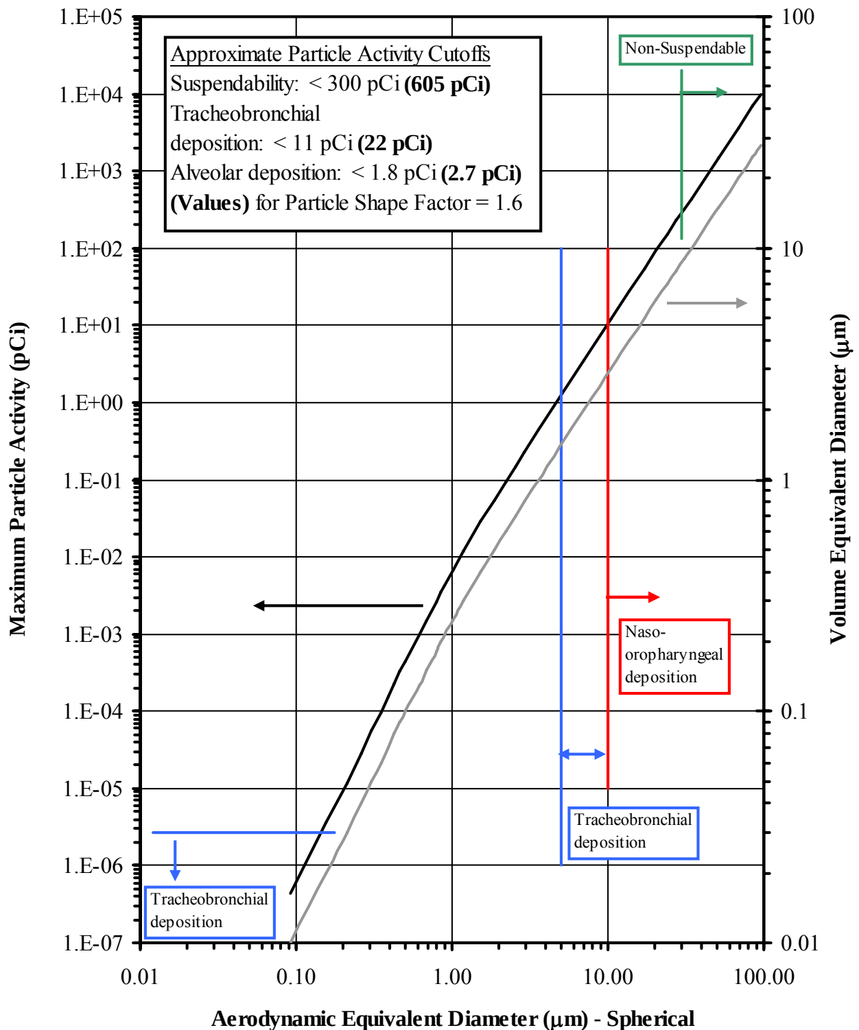
Figure A-14. Maximum Particle Activities and Volume Equivalent Diameters for Aerodynamic Equivalent Diameter (Spherical) \text{PuO}_2 Particles.
