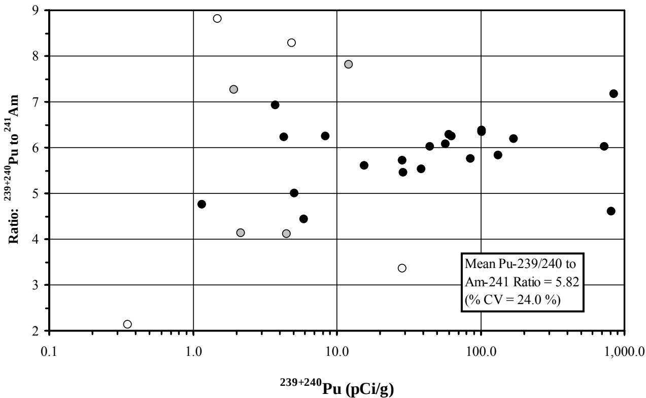
Figure A-4. ^{239+240}\text{Pu} to ^{241}\text{Am} Ratio vs. ^{239+240}\text{Pu} \alpha -Spectroscopy [Data from Duratek (2006)].
