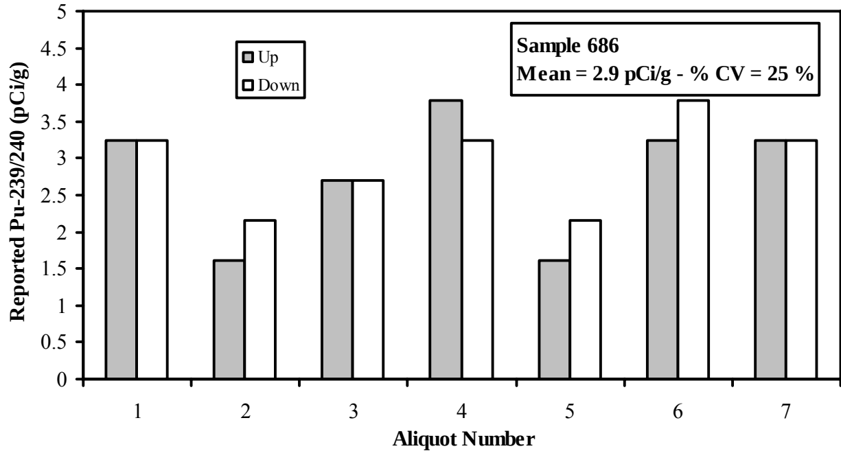
Figure A-7. ^{239+240}\text{Pu} Activity Concentrations of Individual Aliquots (Rademacher 2001).
