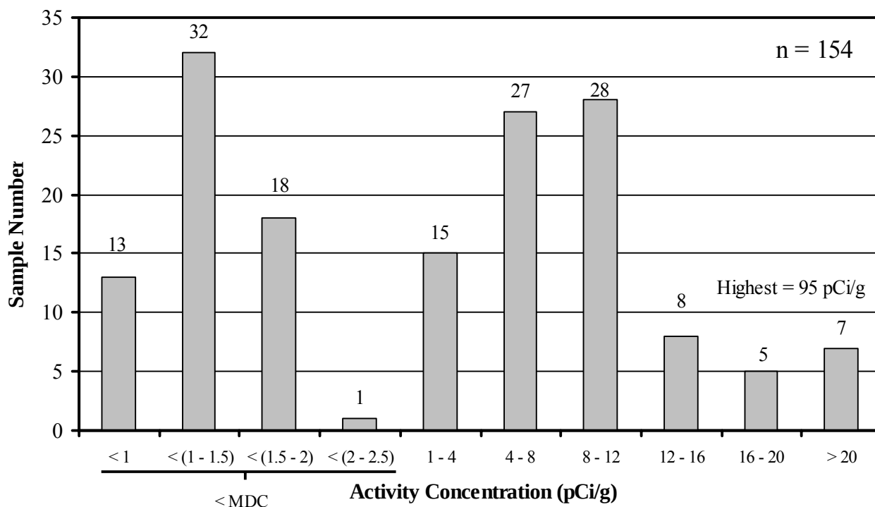
Figure A-13. Elevated Measurement Comparison Final Status Survey ^{239+240}\text{Pu} Activity Concentration Histogram [Data from Duratek (2006)].
