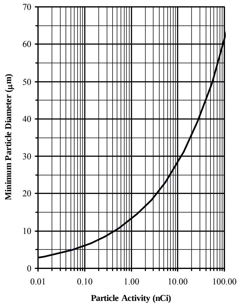
Figure A-8. Minimum ^{239+240}\text{PuO}_2 Particle Diameter, Assuming Spherical, and \rho = 11.5 \text{ g/cm}^3 (Low Range).
