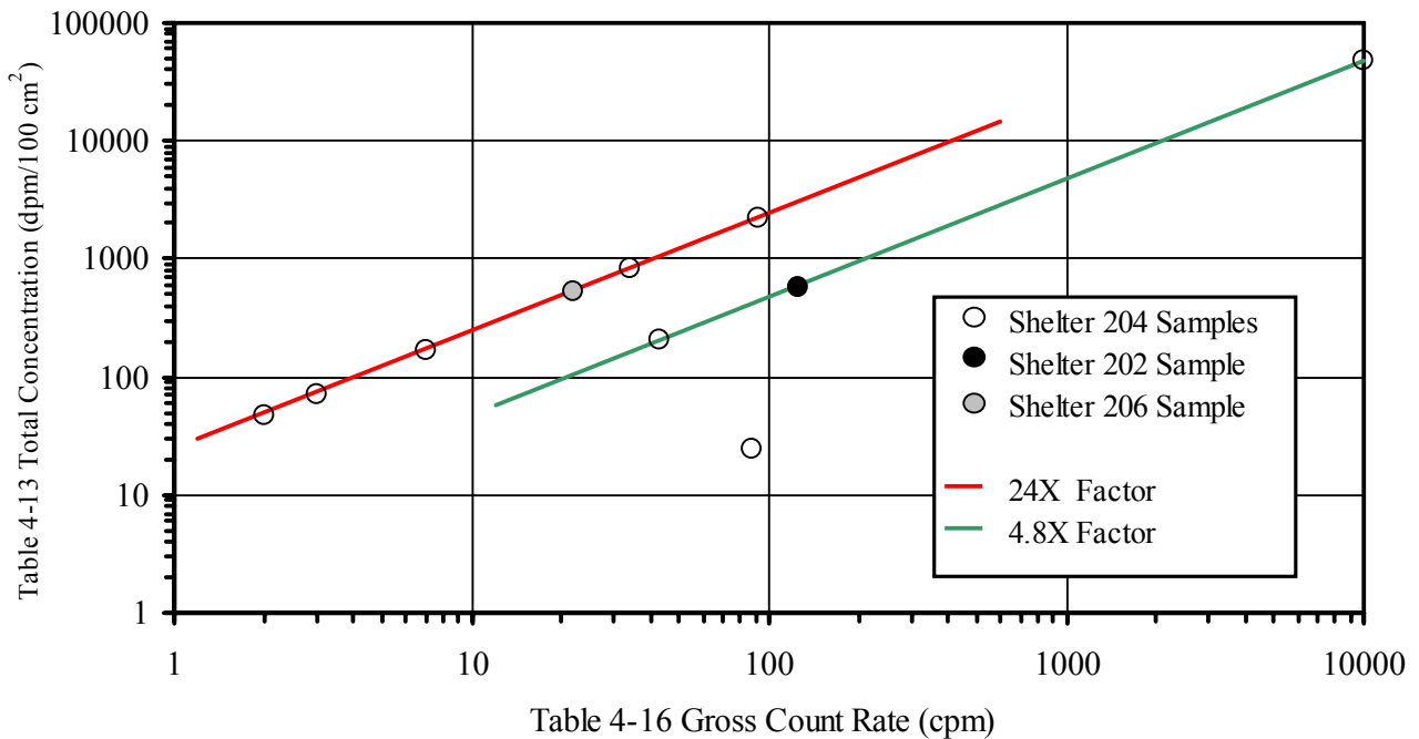
Figure A-19. Scatterplot of Calculated Gross Contamination Concentration (Table 4-13) vs. Reported Instrument Count Rate (Table 4-16) from RI/FS (Earth Tech 1992).
