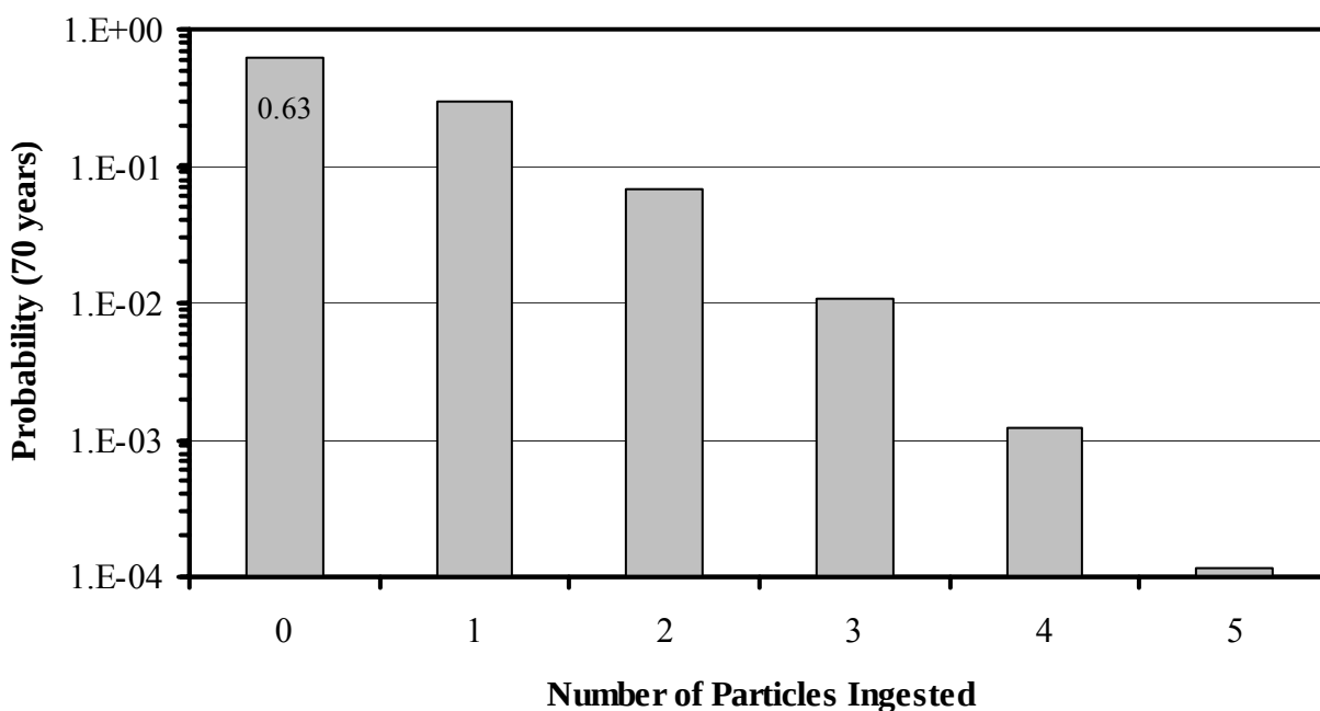
Figure 2-1. Seventy-Year Probability of Ingesting 17 nCi Particles.
