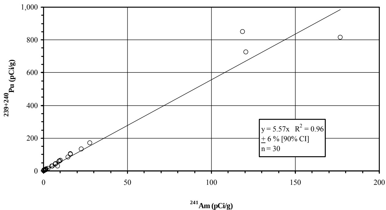
Figure A-3. ^{239+240}\text{Pu} vs. ^{241}\text{Am} \alpha -Spectroscopy [Data from Duratek (2006)].
