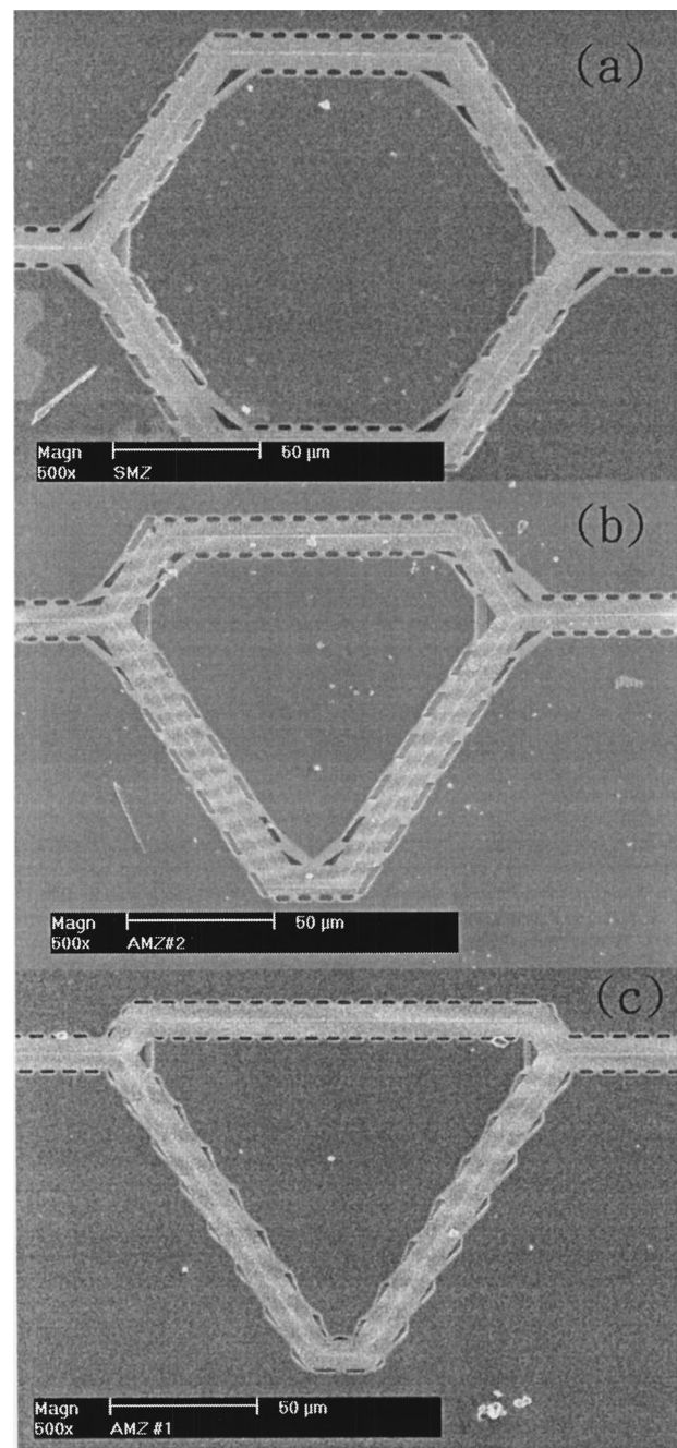
FIG. 3. SEM images of the Mach-Zehnder PCWG with path-length differences of: (a) 0 μm, (b) 75 μm, and (c) 121 μm.
