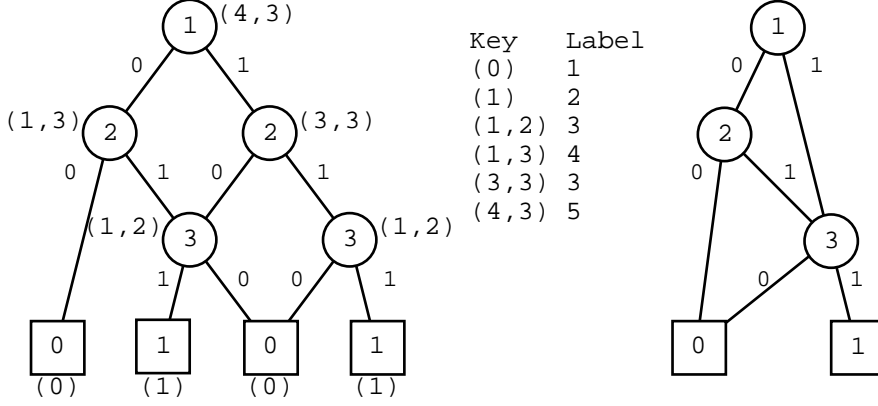
Figure 5.Reduction Algorithm Example
