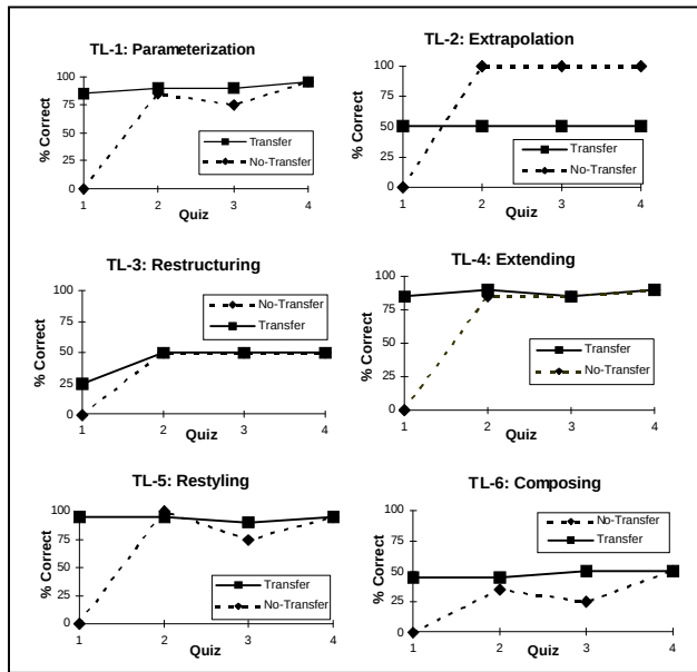
Figure 4: Experiment Results
