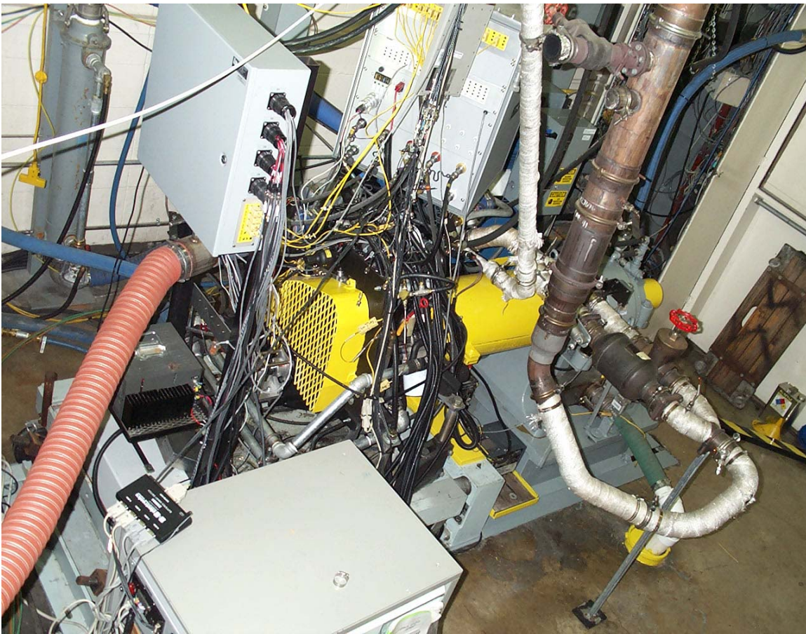
Figure 4. Camless VW 1.9L TDI Engine Test Stand with Integrated Valve and Engine Controllers
