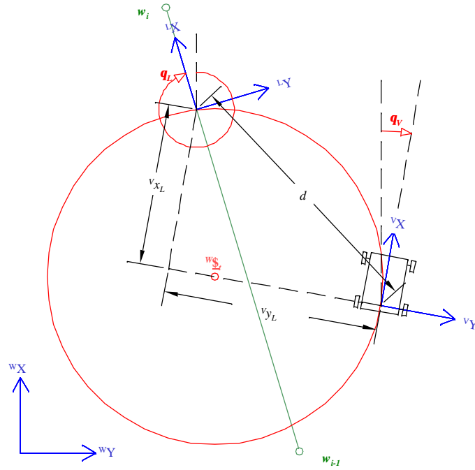
Figure 3.8: Instantaneous Screw for Translating to Look-ahead Point.
