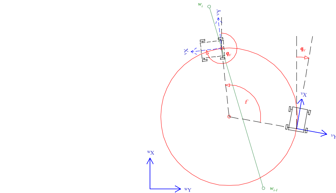
Figure 3.9: Rotation defined by \mathcal{S}_i Instantaneous Screw.
