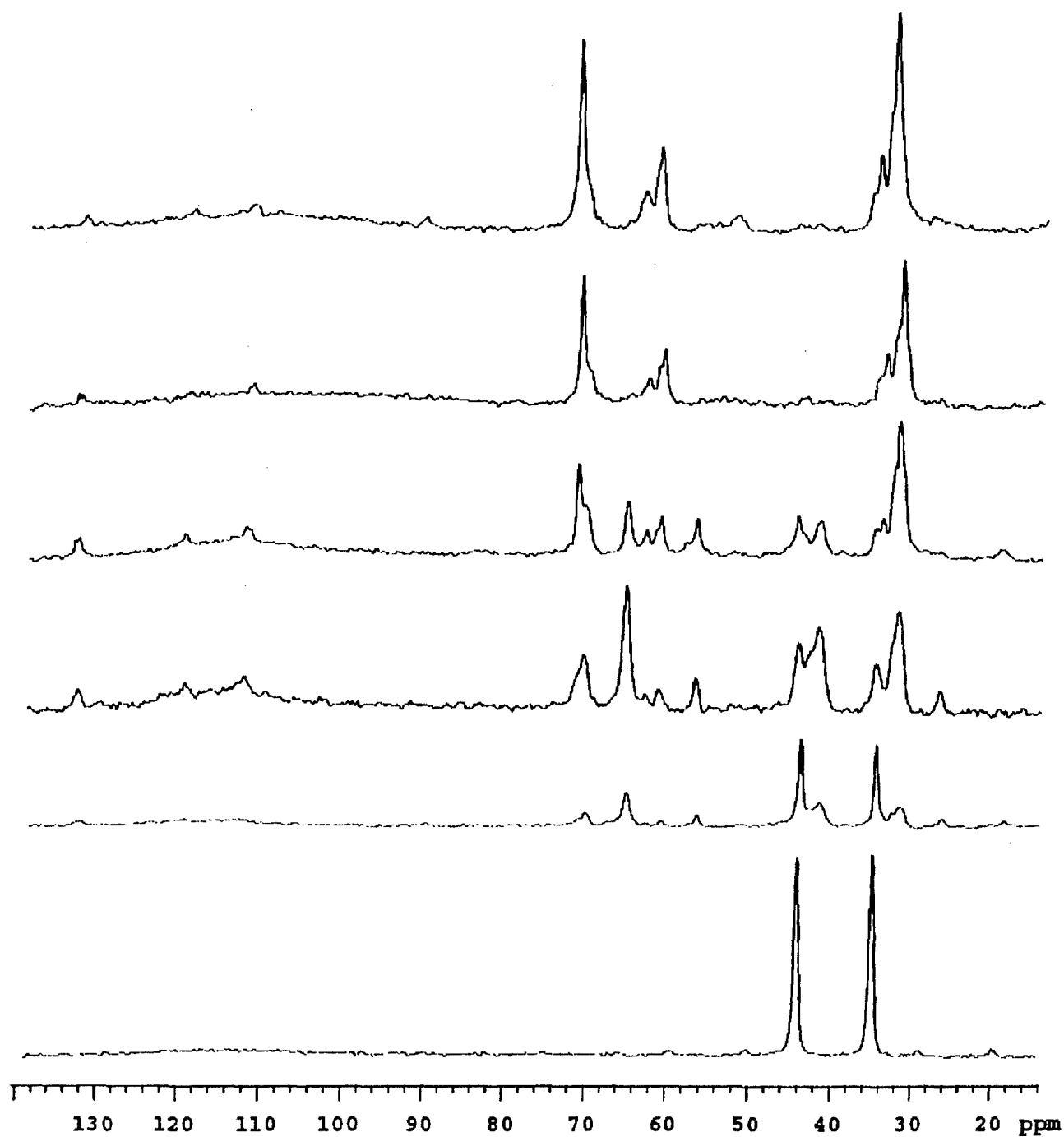
Figure 11. ^{13}\text{C} SSMAS NMR spectra of HD* and water on concrete C03: spectra from bottom to top were acquired at 1 hr, 6 days (shown at 1/5 magnification), 11 days, 44 days, 45 weeks and 62 weeks.
