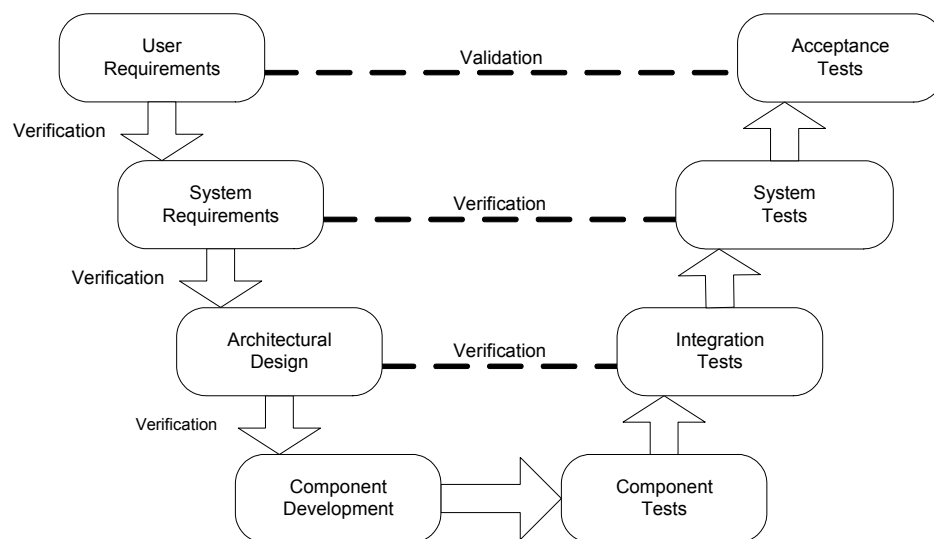
Figure 1: The V-Model
