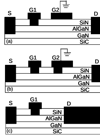
Figure 1. Cross Section of AlGaIn/GaN devices investigated: (a) dual-gate HEMT with single-recess (DG-SR), (b) dual-gate HEMT with double recess (DG-DR), (c) single-gate (SG) HEMT (control device).
