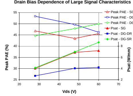
Figure 6. Drain bias dependence of key large signal parameters versus V_{ds} .
