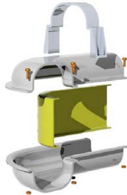
Figure 3.5. Rapid manufacturing design: An example of reducing part count from 16 parts to 1 part. (Courtesy, Loughborough University Rapid Manufacturing Research Group)
