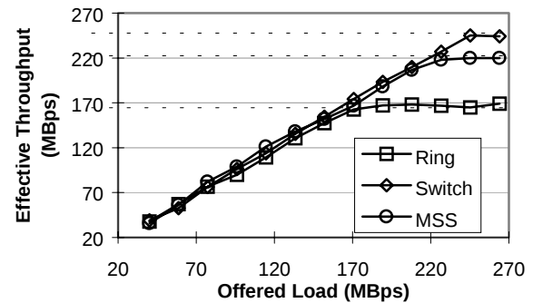
Figure 11: Random Scenario Throughput Results
