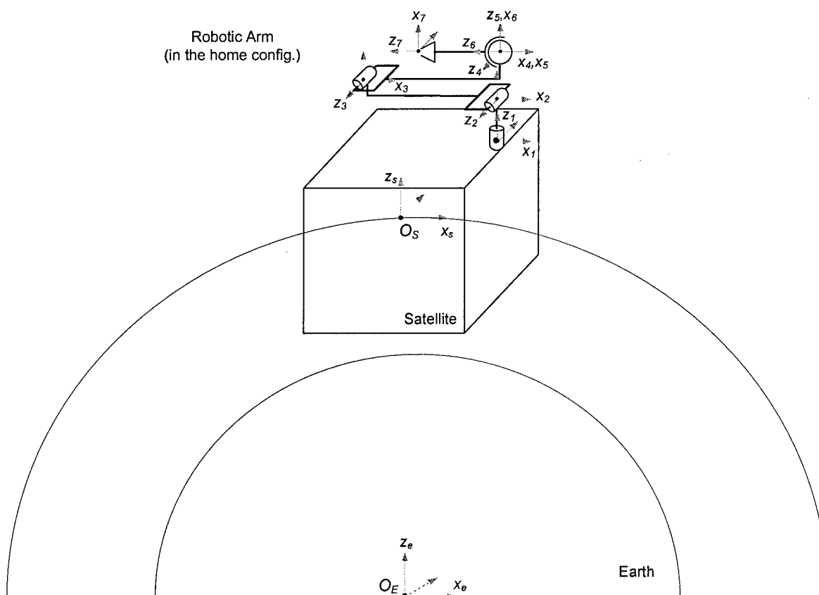
Fig.7 Reference frames of the spacecraft and robotic arm in home configuration
