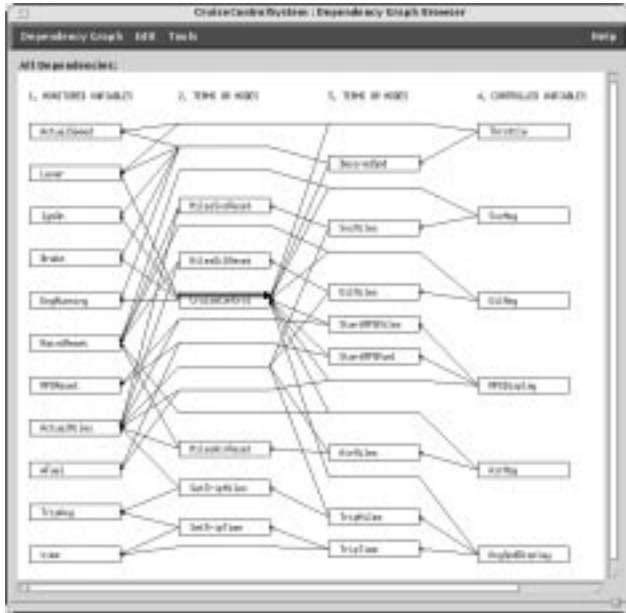
Figure 9. Dependency Graph of Complete Cruise Control.
