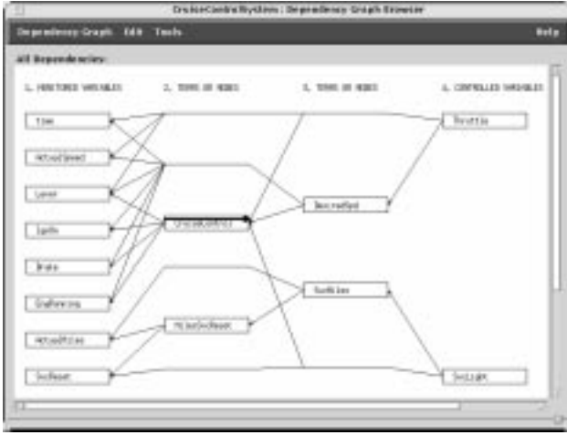
Figure 6. Dependency Graph.
