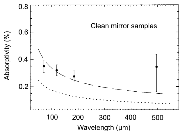
Fig. 6. Measurements and estimated uncertainties for the clean mirror samples. Because there were no significant differences in the measurements for the two clean samples, the average values are shown. The dotted curve is the absorptivity expected for a pure aluminum mirror based on the Hagen–Rubens 11 formula and the resistivity 12 of aluminum at 77 K. The dashed curve shows the best fit to the data, excluding the measurement at 496\ \mu\text{m} , with resistivity taken as a free parameter (see text).
