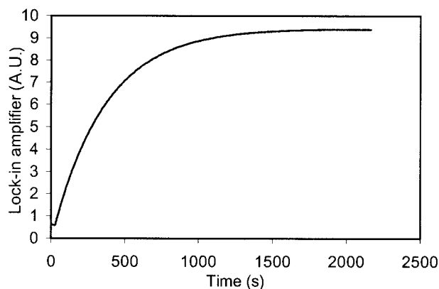
Fig. 5. Typical heating curve for a clean mirror sample at 77 K. The increase in lock-in amplifier signal corresponds to a temperature rise of \sim 300 mK with a thermal time constant of \sim 7 min and has a noise level of \sim 0.6 mK (rms).
