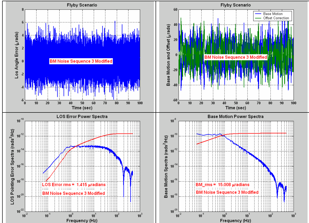
Figure 17 Strapdown configuration responses for angular disturbance base motion sequence 3 from Figure 2. For a base motion spectra of 15.0 \mu radians rms the resulting line-of-sight error is calculated at 1.42 \mu radians rms. Base motion sequence 3 has a significantly lower rms magnitude than sequence 1 and slightly lower than sequence 2. However, it has the highest line-of-sight error due to the highest magnitude of energy at high frequencies.
