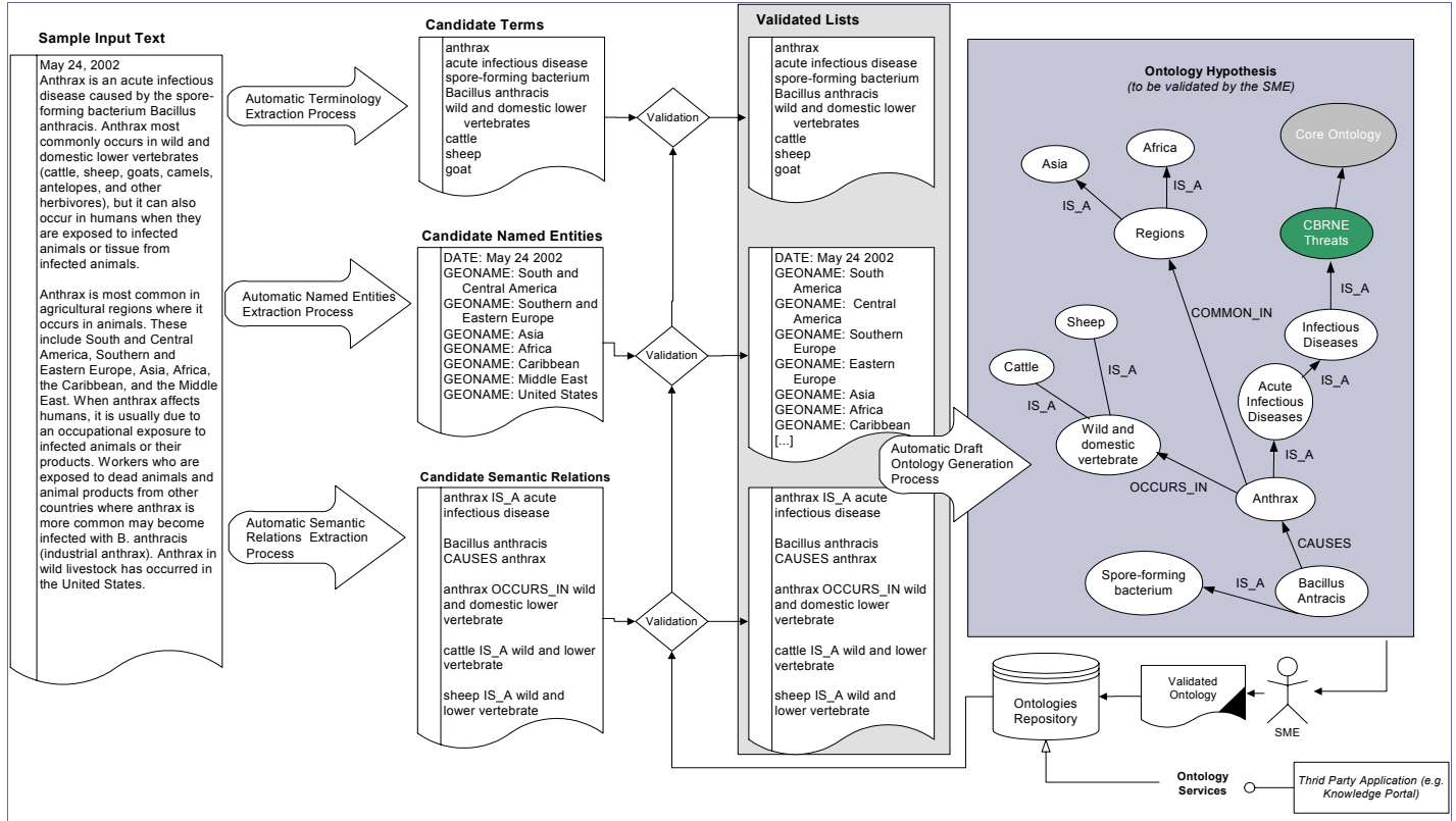
Fig. 9: Turning Electronic Texts into Domain Ontologies Using the SACOT Framework
