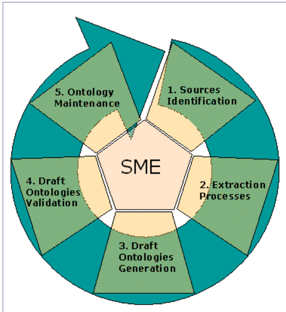
Fig. 2: SACOT's Ontology Engineering Process
