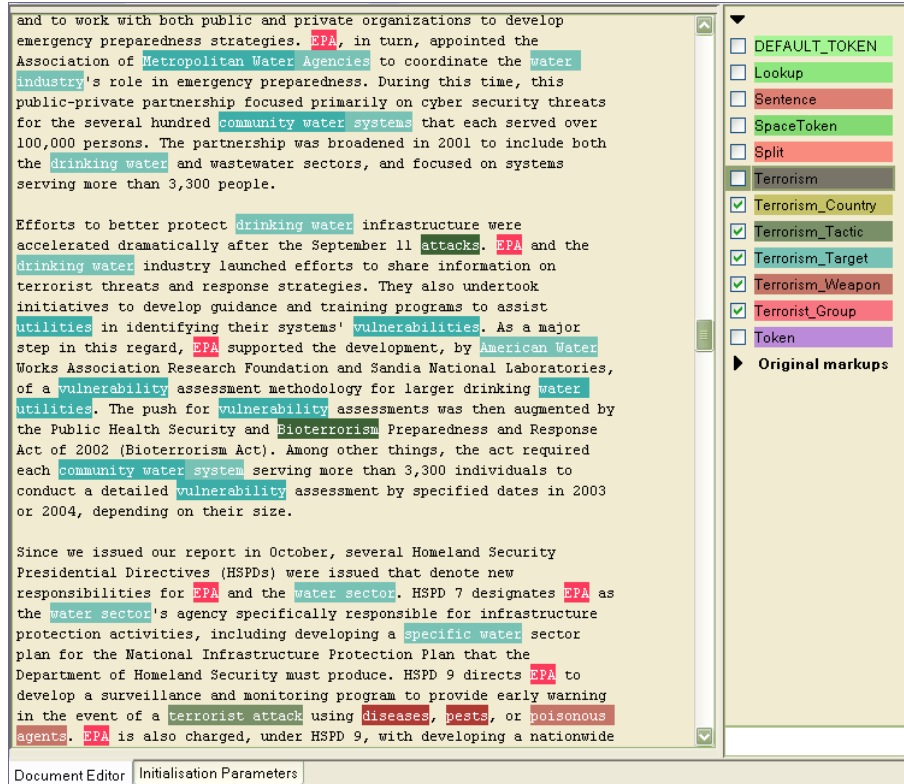
Fig. 4: SACOT's Terrorism-related Named Entities Automatic Identification Using GATE
