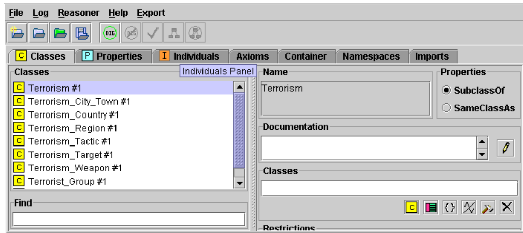
Fig. 3: Partial Terrorism-related Named Entities Ontology
