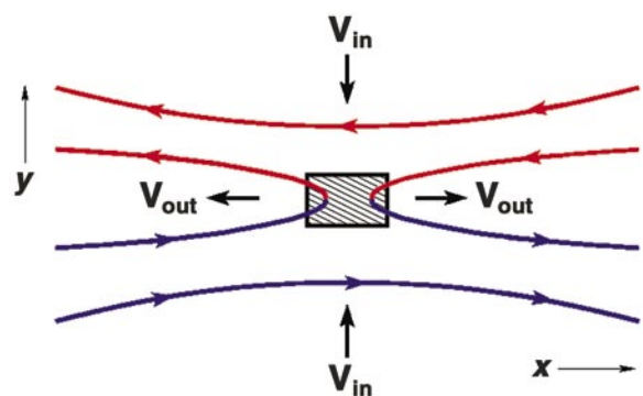
FIGURE 9 Standard, two-dimensional concept of magnetic field line reconnection.
