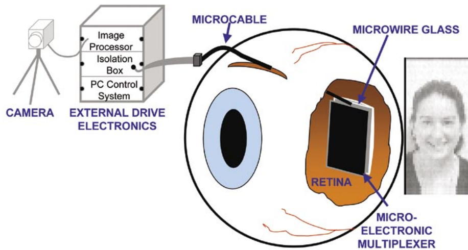
FIGURE 1 Retinal prosthesis test system, illustrating the device positioned against the retina during a one-hour surgical experiment. To provide basic visual function that is sufficient to treat common types of blindness (enough pixels for facial recognition or to read text), an extremely thin microcable passes through an incision in the eye wall, allowing a direct means of powering the device and inputting image data. The image to the right represents the image quality achievable with the 80 x 40 device. A future retinal prosthesis system, now in the planning stage, would be wireless – no microcable required – and backside illuminated.
