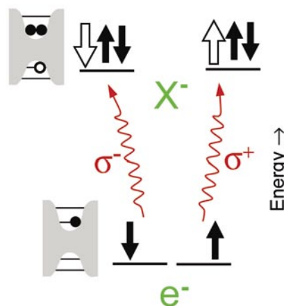
FIGURE 6 Total energy spin configurations of a ground state electron ( e^- ) and its optically excited state (negative trion). Open and filled arrows represent hole and electron spins, respectively. Optical transitions are achieved with right ( \sigma^+ ) and left ( \sigma^- ) circularly polarized light.
