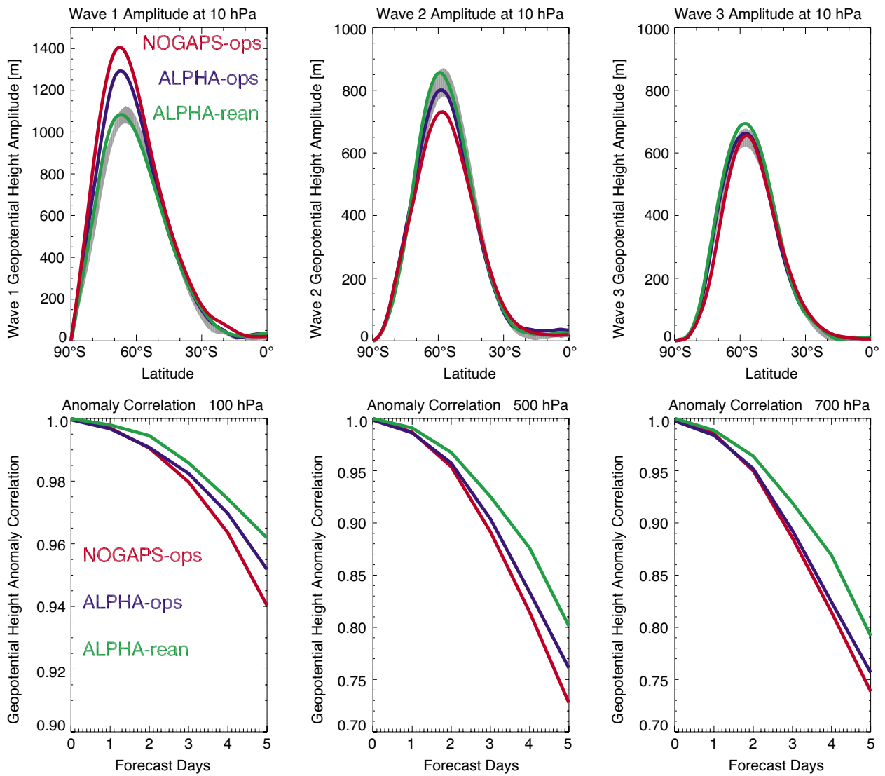
FIGURE 3 (Top row) geopotential height zonal wavenumber 1, 2, and 3 amplitude at 10 hPa on September 25, 2002 (12 UTC) over the SH for three al initialized on even-numbered days from September 18 to October 10, 2002 (12 UTC). The anomaly correlation for each forecast is calculated with the analyses used for initialization.
