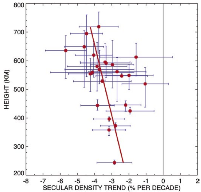
FIGURE 2 Summary of secular density trends derived from 25 objects, as a function of drag-weighted average height (near perigee). The horizontal bars indicate the 1 \sigma uncertainty in the trends, and the vertical bars denote the range of heights covered by each object.
