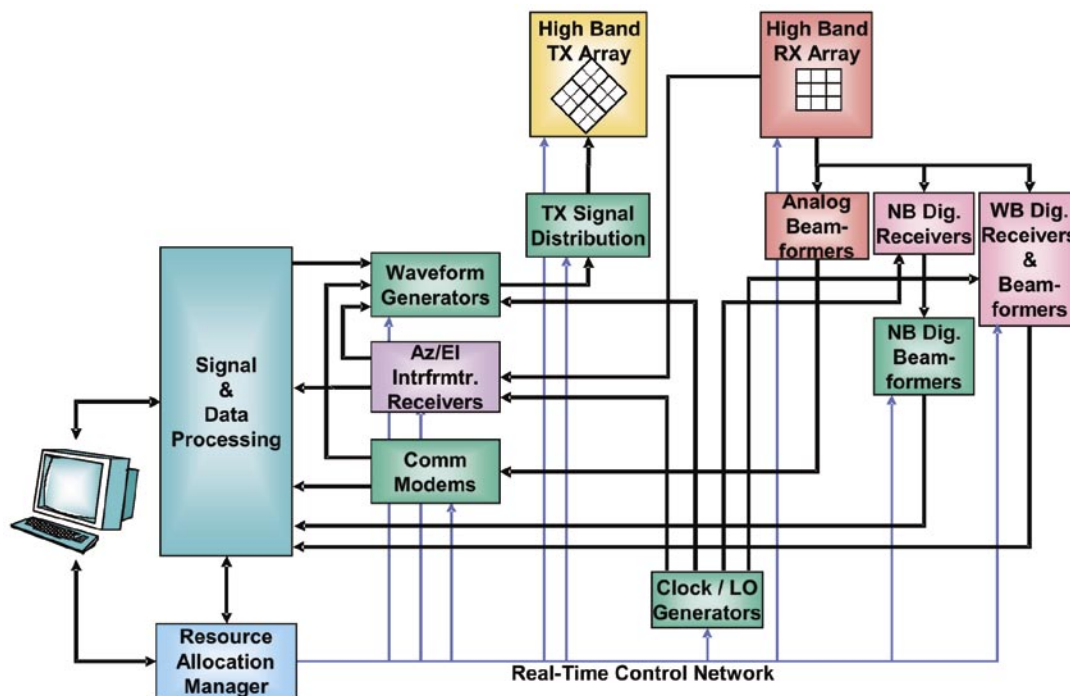
FIGURE 1 AMRFC receive array and transmit array, illustrating selectable partitioning to support RF functions. Difference in angle orientation reflect individual contractor's approach.
