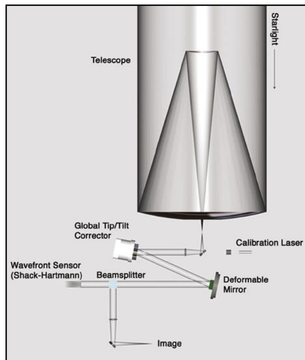
FIGURE 4 Schematic diagram of a generic adaptive optics system.
