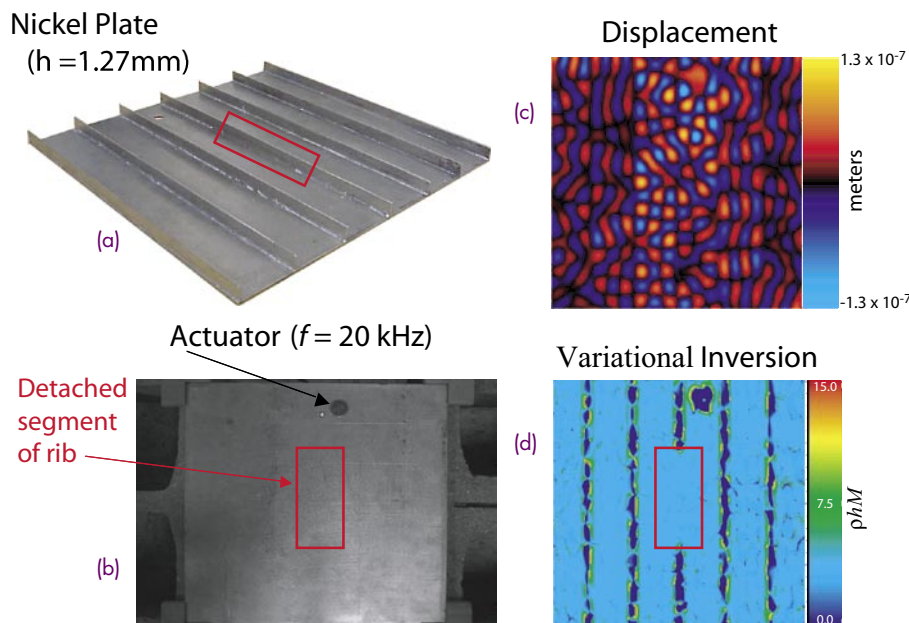
FIGURE 3 Experimental demonstration to detect and locate frame detachment in a rib-strengthened thin nickel plate. (a) Shows the ribbed side of the plate, and (b) shows the external measurement side with the red rectangle marking the hidden location of frame detachment. (c) Shows the SLDV-measured surface displacements caused by a point actuator in contact with the plate excited at 20 kHz, and (d) shows the result of applying the variational flexural inversion algorithm, where the obscured frames manifest themselves by the deep blue lines and the detached region by the absence of such.
