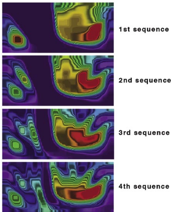
FIGURE 9 Calculations on a 3200 \times 36 \times 80 grid, using computational cells of 2.5 \mu\text{m} , that show stretching and folding indicative of chaotic advection after four sequences in the herring-bone mixer.
