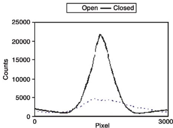
FIGURE 6 Cross cut of the two images in Fig. 5. The solid line is the cross cut of the closed loop image and the dashed line is the cross cut of the open loop image.
