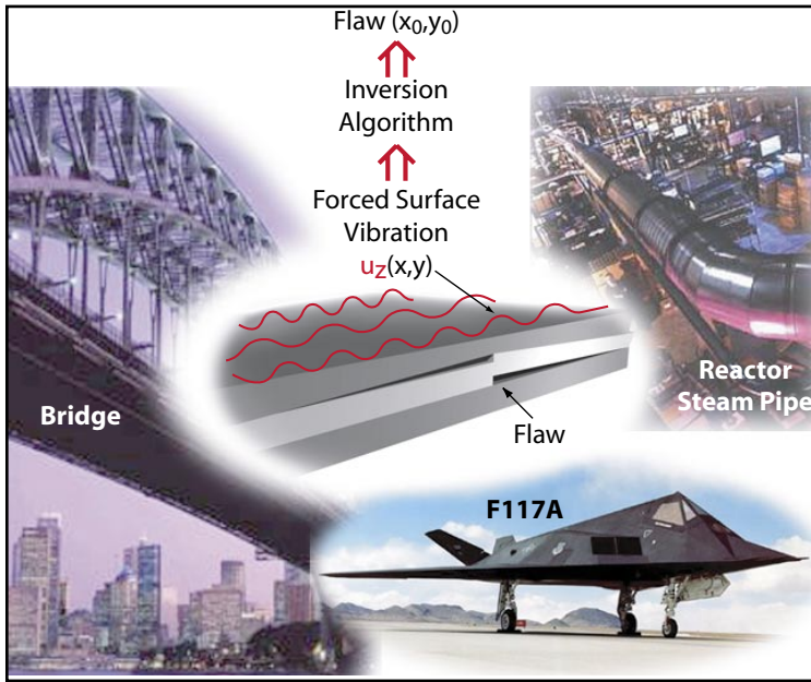
FIGURE 1 Depiction of the structural acoustic fault monitoring methodology applied to a variety of structures. Surface displacements are monitored over the area of interest due to structural vibrations induced either by an applied shaker or an acoustic source. The displacements measured over the surface are algorithmically inverted to produce a map of a desired material parameter that serves to detect and locate the flaw.
