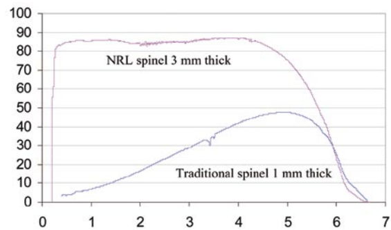
FIGURE 3 NRL spinel transmits within 1% of the theoretical bulk transmission throughout its range, while the traditional spinel has poor transmission resulting from scattering losses.
