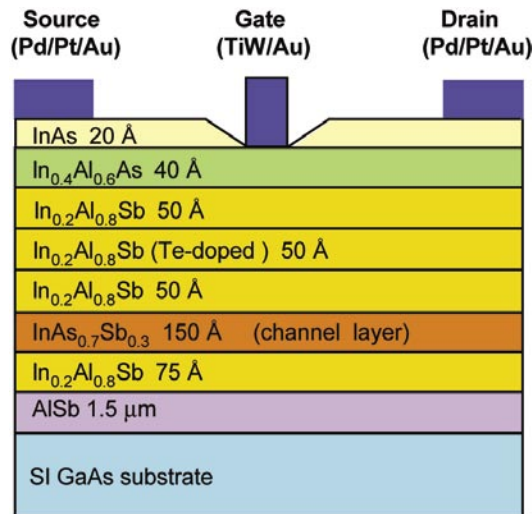
FIGURE 8 Cross section of the 6.2 Å InAlSb/InAsSb HEMT layer design.
