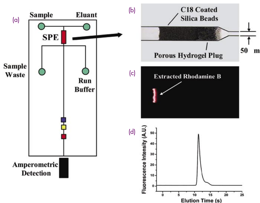
FIGURE 1 (a) SPE microchip design; (b) close-up of packed bed; (c) fluorescence microscope image of Rhodamine B loading onto packed bed; and (d) electropherogram for micro-SPE of 100 \mu\text{M} Rhodamine B.
