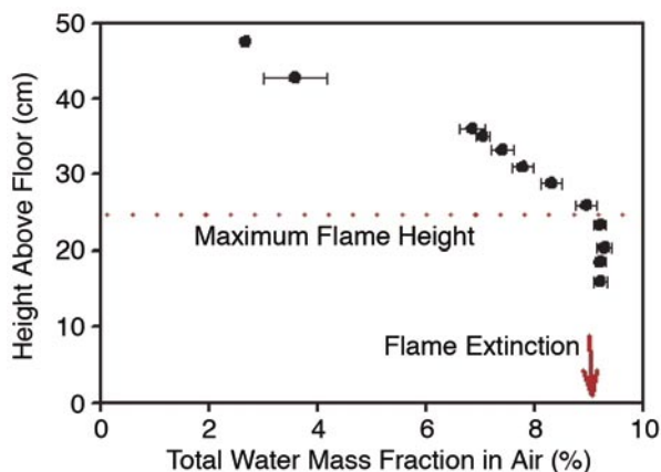
FIGURE 5 Height in corral vs water mass fraction (very fine water mist and vapor). Flame extinction studies show that very fine water mist achieves the theoretical quantitative flame extinguishing potential for water in this environment based on a thermal fire suppression mechanism.
