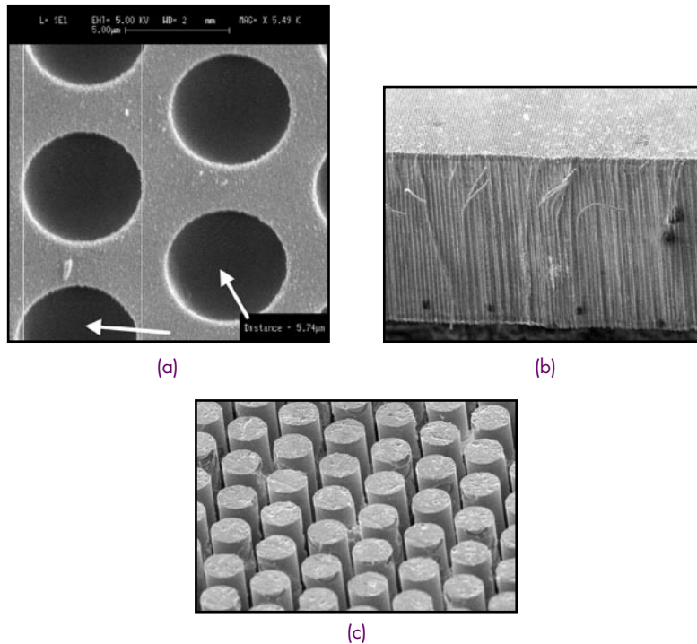
FIGURE 4 Various stages of microwire glass fabrication: (a) an SEM of the microchannel plate starting material — typical channel diameters are 5 \mu\text{m} with center-to-center spacings of 8 \mu\text{m} ; (b) SEM of a cleaved edge of a nickel-filled sample — channel lengths can be plated up to one millimeter; (c) SEM view of top surface showing microwires protruding from the glass after etch-back.
