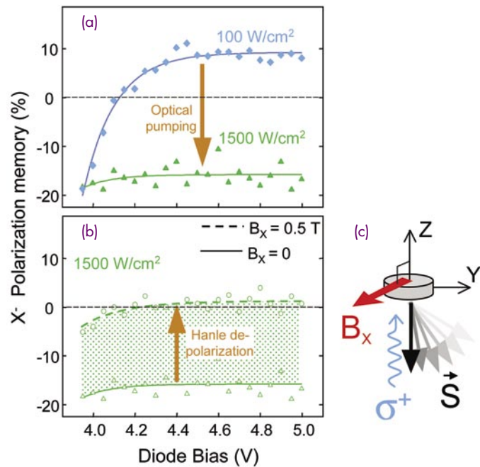
FIGURE 8 (a) Polarization memory of negative trion ( X^- ) for two laser excitation intensities. (b) Elimination of negative polarization memory for X^- through Hanle depolarization of optically pumped electrons. (c) Geometry of Hanle effect: optically pumped electrons are initially oriented parallel to Z axis, but are depolarized by precession about transverse magnetic field B_x .
