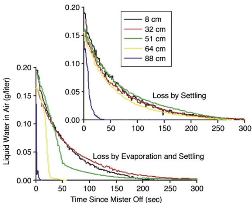
FIGURE 6 Fine water mist drop density decay time as a function of height. At least two competing loss mechanisms occur for the mist: settling and evaporation. The evaporation loss is rapid, until the surrounding environment becomes saturated with water vapor, then the slower settling mechanism dominates.
