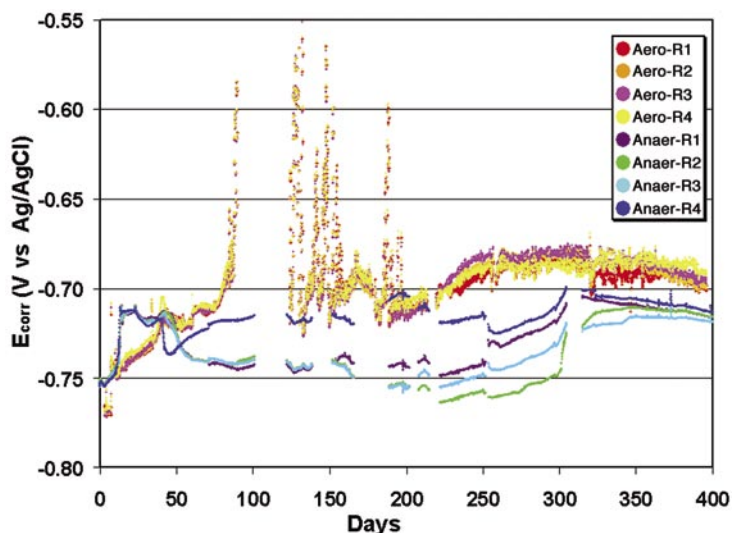
FIGURE 11 Average E_{\text{corr}} (vs Ag/AgCl) over time values for C1020 samples in stagnant aerobic (aero) and anaerobic (anaer) conditions displayed by row (R). R1, R2, R3 – vertically orientated samples, with R1 being at the top of the tank, R3 toward the bottom, and R2 between the two. R4 – horizontally orientated sample at the bottom of the tank.
