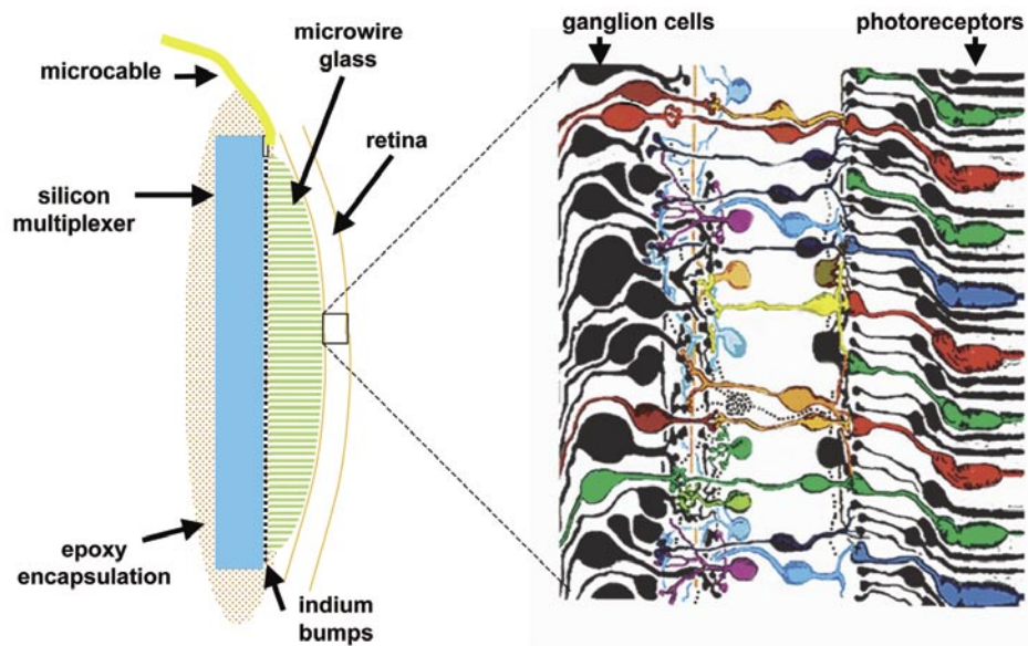
FIGURE 2 Device architecture and the corresponding retinal anatomy with regard to device placement. Note that the outermost layer of the retina consists of photoreceptors and the ends of the micro-wire glass are positioned in close proximity to the ganglion cell layer of the retina.
