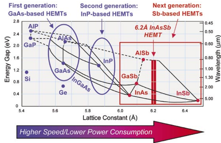
FIGURE 7 Energy gap vs lattice constant chart showing high-speed, low-power semiconductor trend in HEMT technologies.
