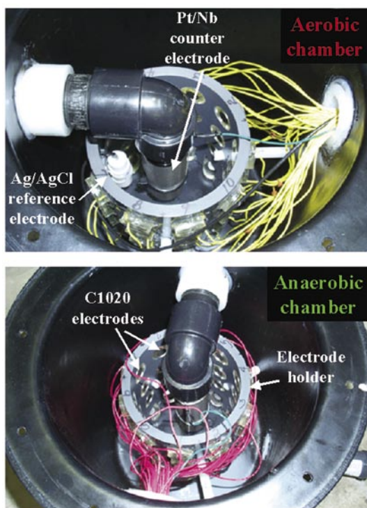
FIGURE 10 Heavy gauge plastic experimental chambers each containing Ag/AgCl reference electrode, Pt/Nb mesh counter electrode, cylindrical electrode holder, and 36 individually addressable C1020 electrodes (27 vertically orientated, 9 horizontally orientated).
