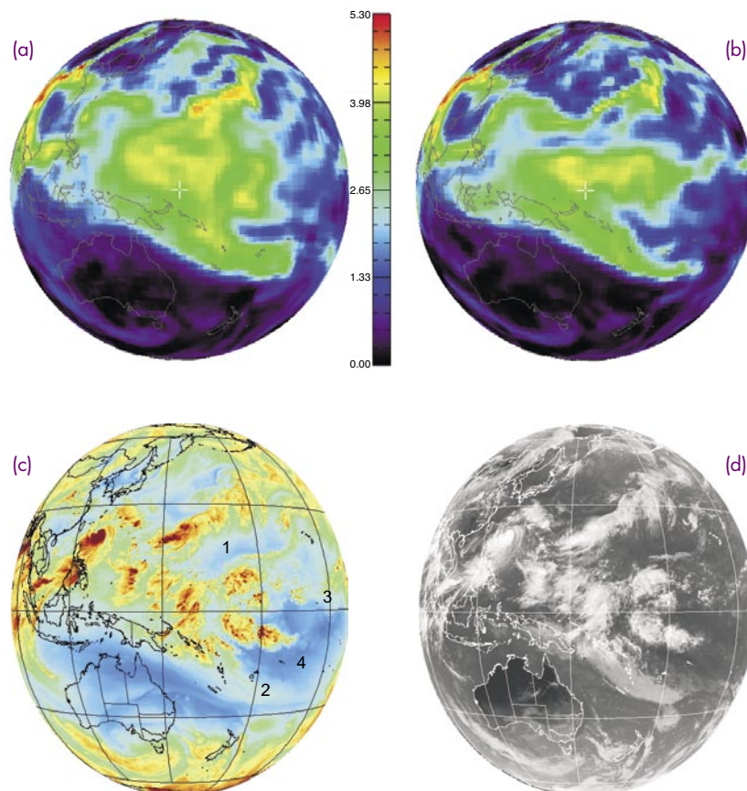
FIGURE 3 (a) Analyzed 500 hPa specific humidity ( \text{g kg}^{-1} ) at 06Z on August 10, 2004, control run; (b) AMSU-B run; (c) GOES-9 6.7 \mu\text{m} water vapor channel image at 0525Z; (d) GOES-9 infrared image at 0525Z. Features improved in the AMSU-B run include (1) dry channel north of the Intertropical Convergence Zone (ITCZ), (2) sharp feature at tail of South Pacific Convergence Zone, (3) sharp gradient in ITCZ, and (4) shape of dry region in Central Pacific.
