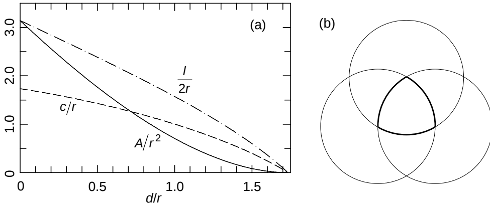
Figure 10: (a) Area A , chord lengths c and perimeter l of an equilateral circular triangle (equal radii and equal separations of circle centres) as a function of the ratio d/r of separation to radii. (b) An equilateral circular triangle (thick lines) with d = r .
