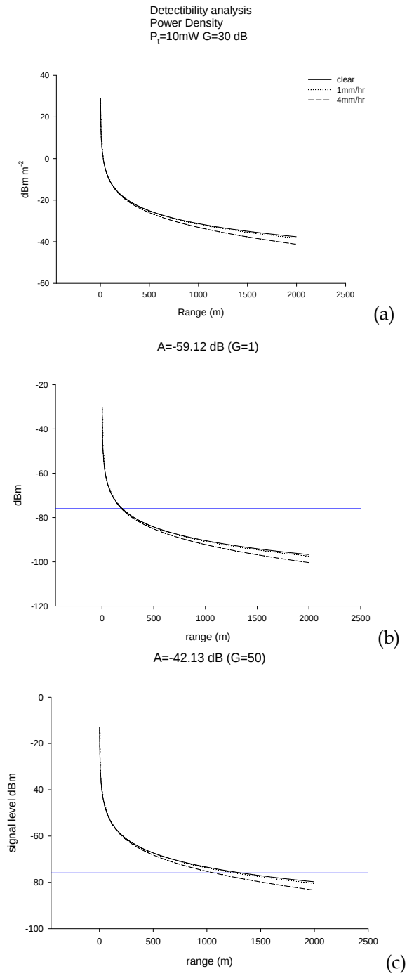
Figure 7: Target detectability by receiver at standoff distance from transmitter a) power density for ERP=10\text{ W} signals, b) signal level G_r=1 and G_r=50 . The blue line shows receiver system noise level \sim -75\text{ dBm} .
