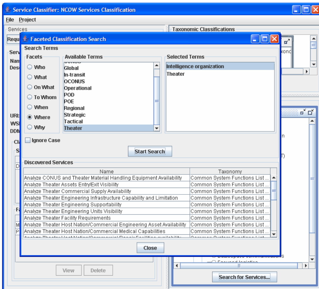
Figure 5. Service Discovery by Faceted Classification
