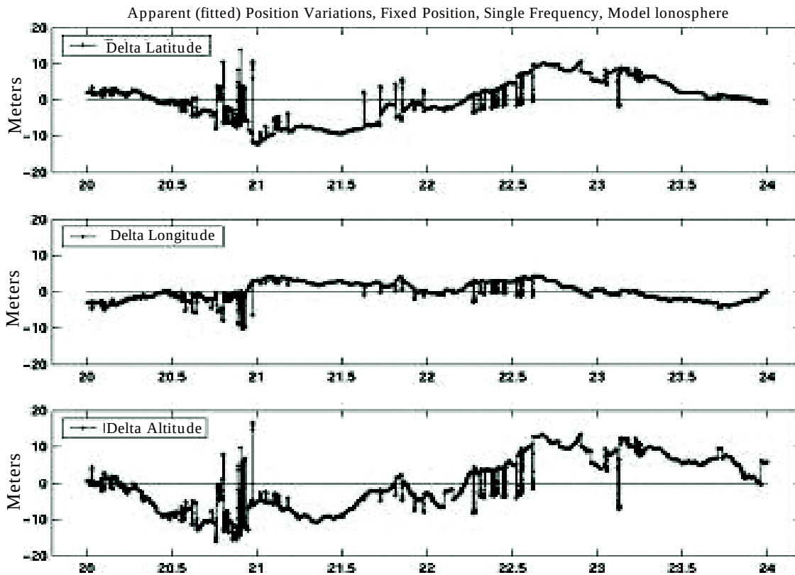
Fig. 10. Position components estimated by the stationary single-frequency receiver. Effects of ionosphere include the rapid spikes and the long-term variations in the position. The altitude variations are anticorrelated with the timing variations of Fig. 8
