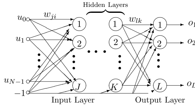
Figure 3: Multi-layer perceptron.
