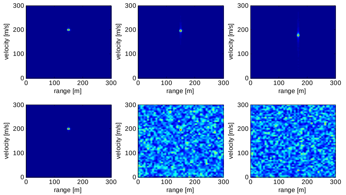
Figure 9: Range-Doppler profiles. Radars operate with the following relative transmit powers: +40 dB, +3 dB and 0 dB. Upper row: radar returns of the first, second and third radars without ML. Lower row: radar returns of the first, second and third radars with ML.
