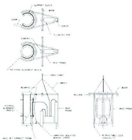
FIG 1 WHIC SLED CONFIGURATION
