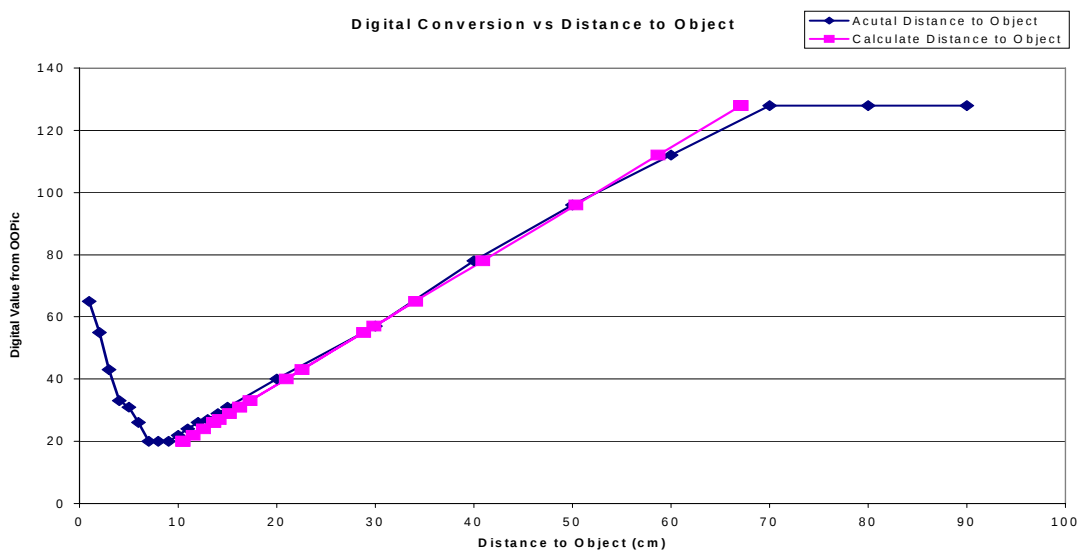
Figure 28. OOPic Digital Conversion versus Distance to Object for IR Ranger.
