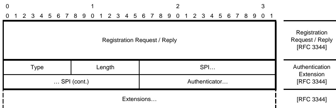
Figure 21. Authentication Extension (After: [4]).
