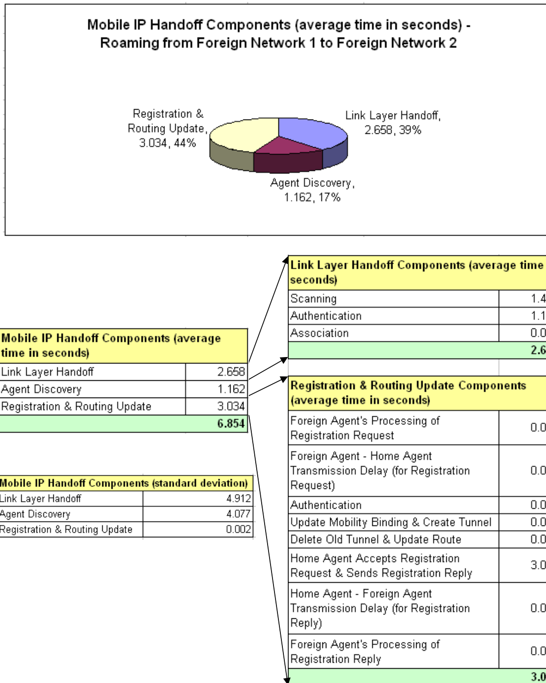
Figure 44. Mobile IP Handoff Performance Statistics for Roaming from Foreign Network 1 to Foreign Network 2.
