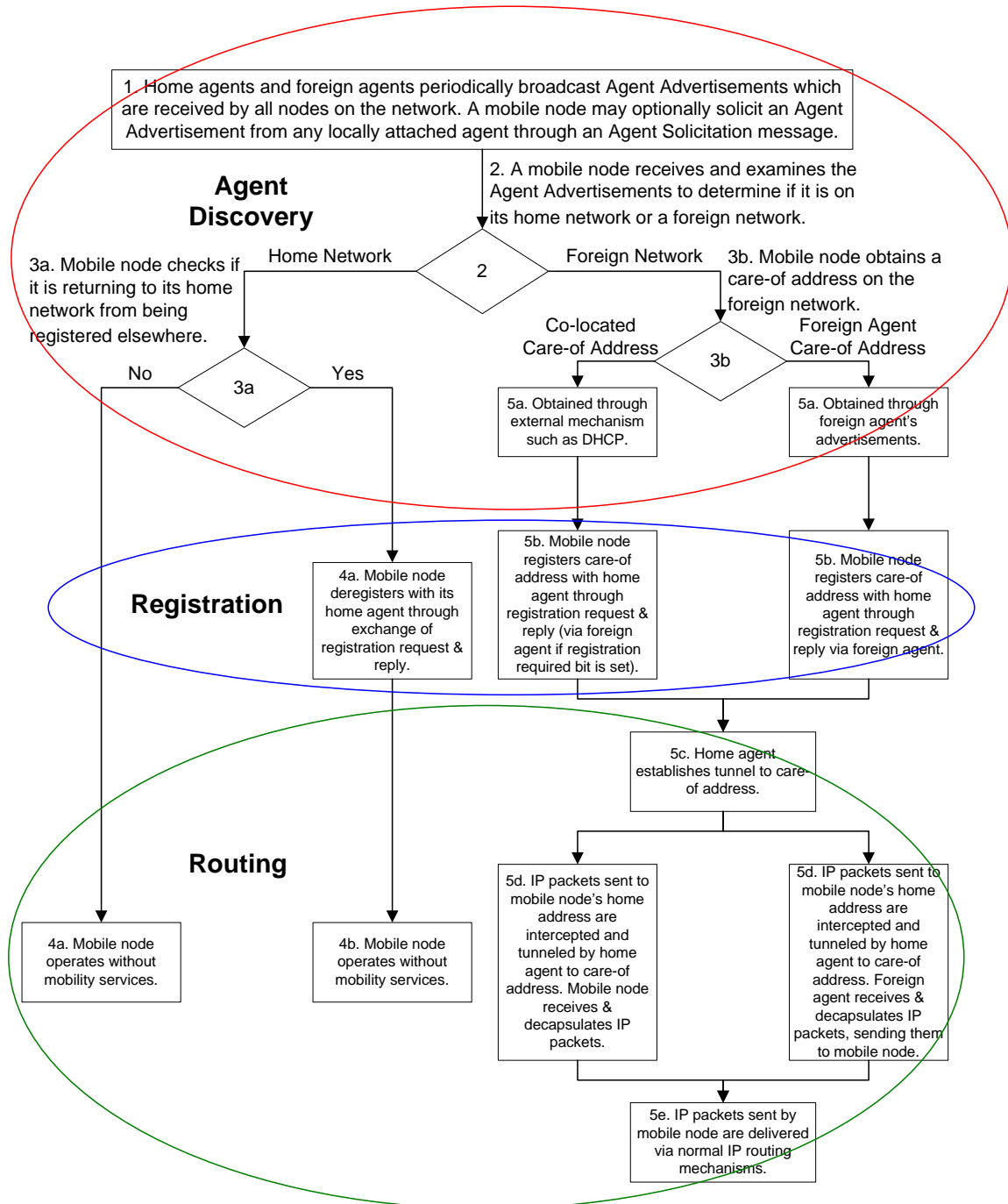
Figure 2. Overview of Mobile IP Operation.
