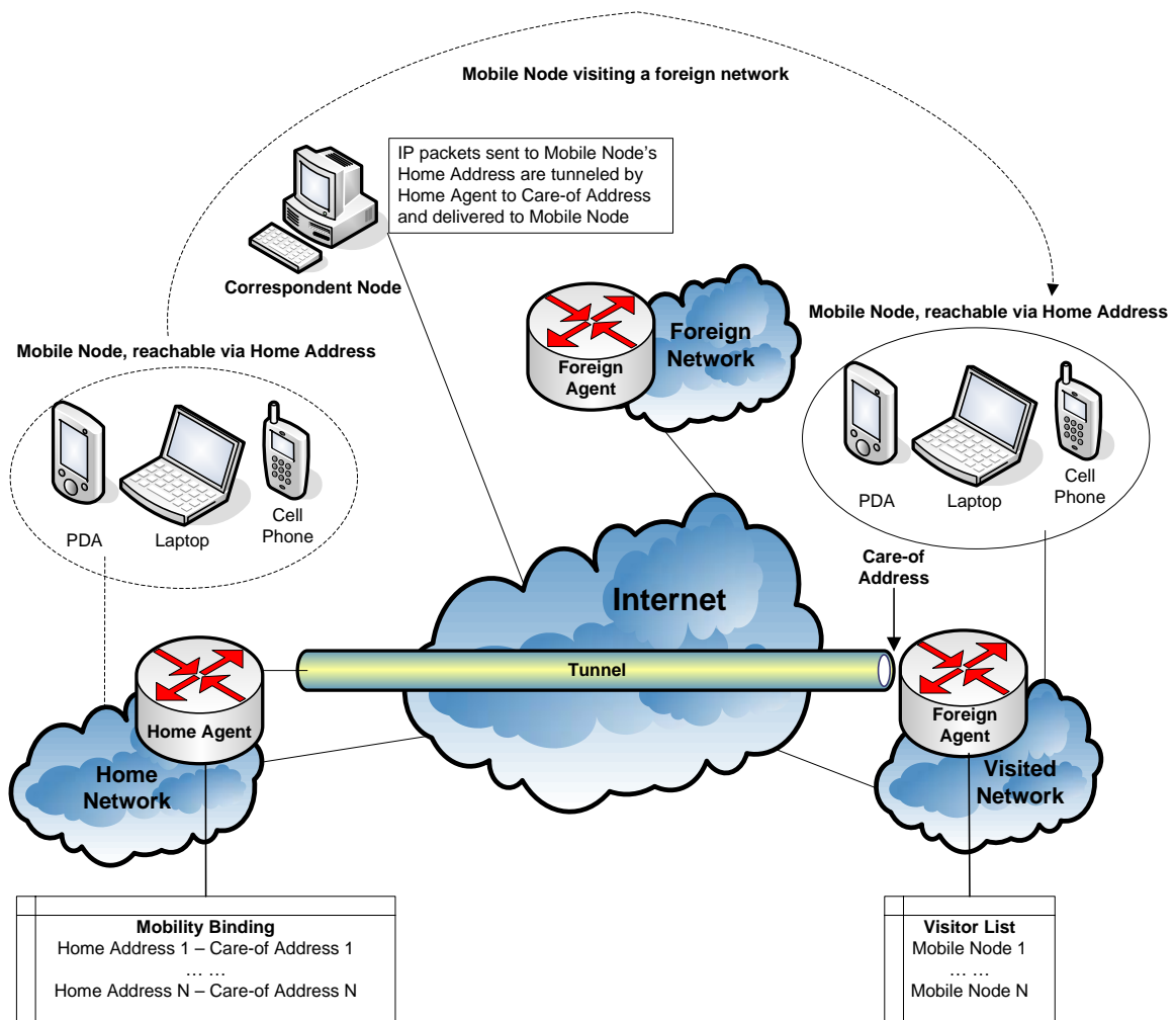
Figure 1. Mobile IP Entities and Relationships (After: [5] & [6]).
