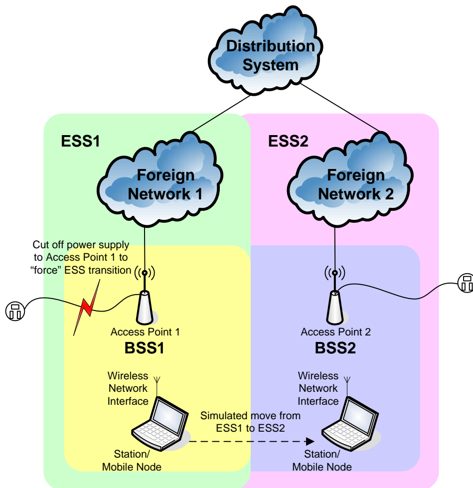
Figure 34. IEEE 802.11 Wireless Network in Devoted Setup.
