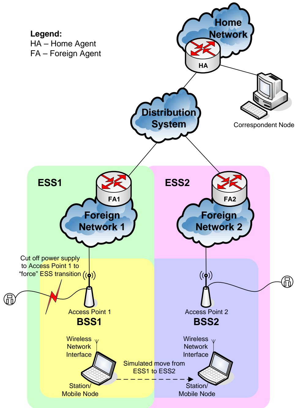
Figure 35. Mobile IP Version 4 Network in Deviced Setup.
