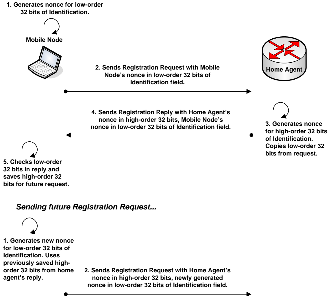
Figure 23. Replay Protection using Nonce.
