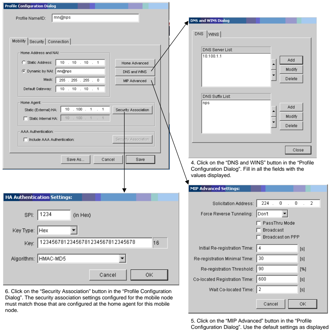
Figure 56. Mobile Node's Configuration.
