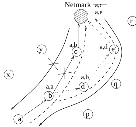
Figure 2. Setting up of paths between netmarks and other nodes
